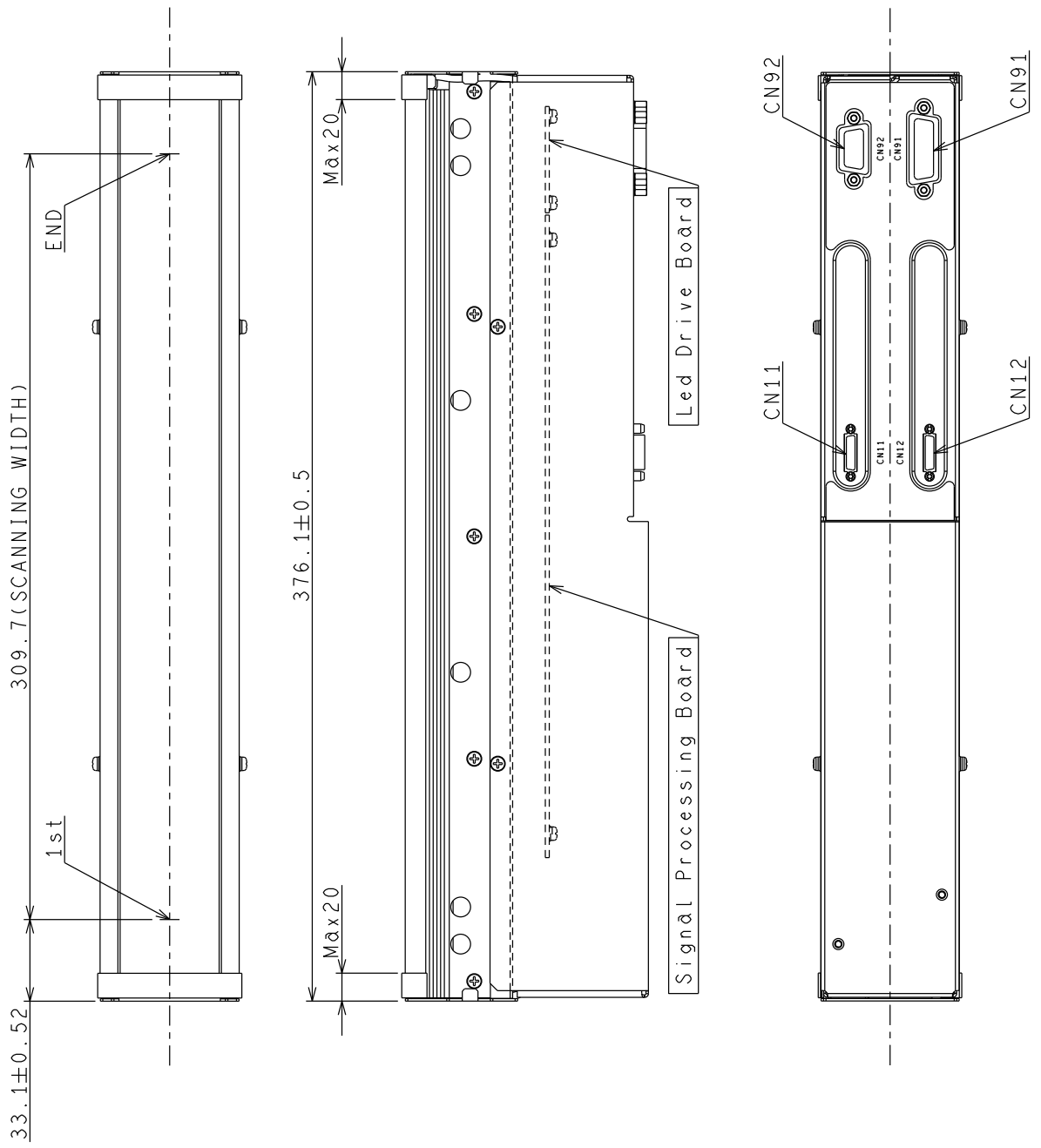
KD6R309MX Outline drawing
