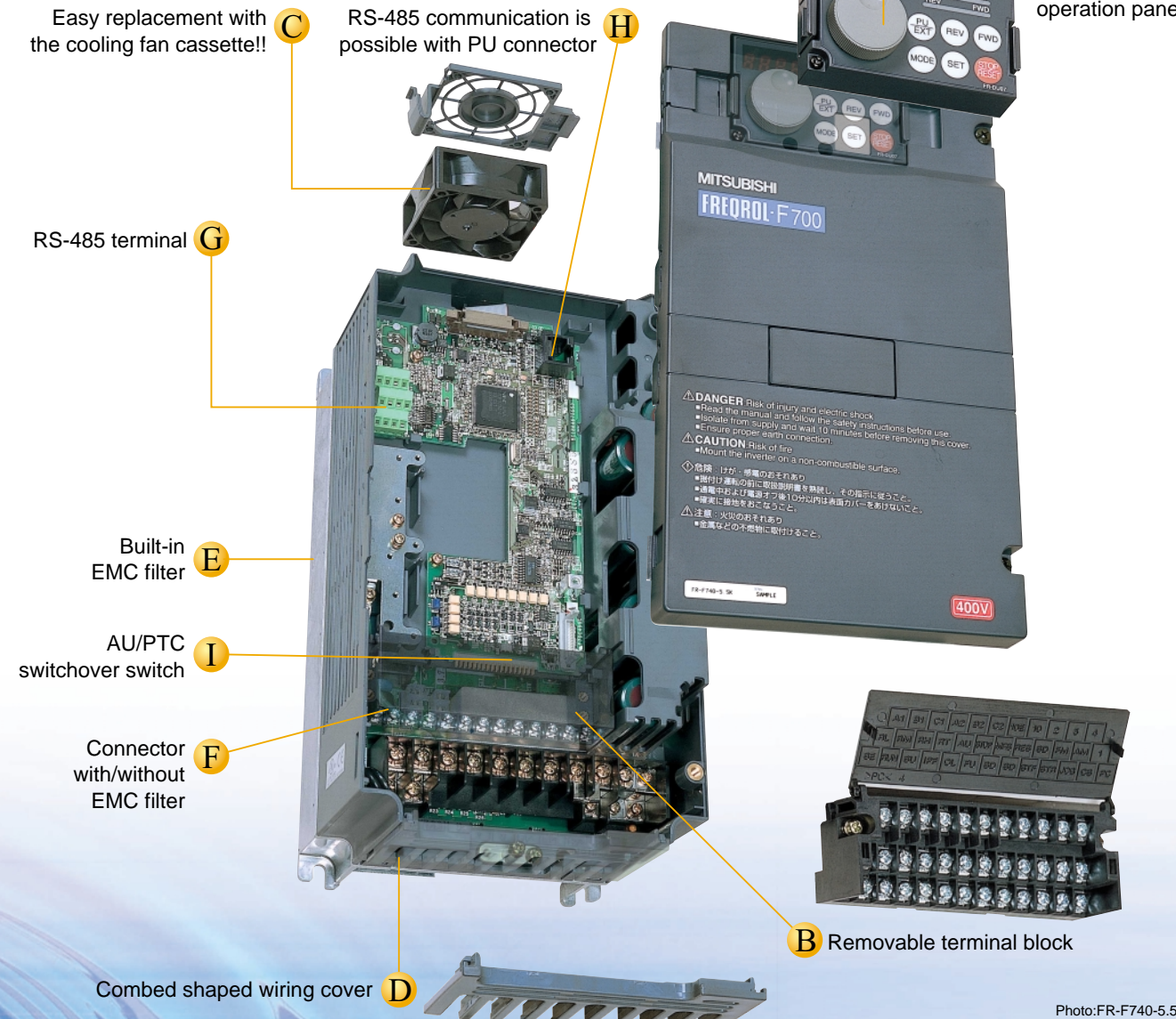
Photo:FR-F740-5.5K
