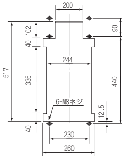
FR-A7CN04
