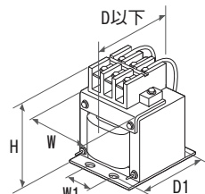
FR-HEL-3.7K~55K FR-HEL-H0.75K~H55K
