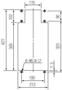
FR-A7CN03
