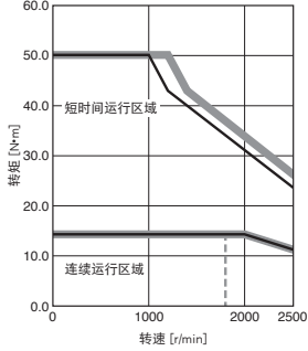
HK-ST3024WJ 转矩提升
