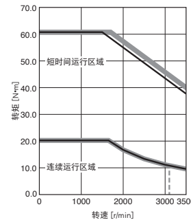
HK-ST3524WJ 转矩提升
