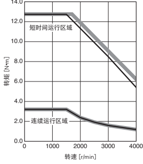
HK-ST524WJ 转矩提升
