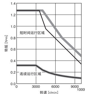
HK-MT13VWJ 转矩提升
