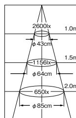
JRS12V50W-FL/BS
