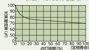
図2 HCI®-TE, TC, TC/E, T (HCI®-TE100Wを除く)
