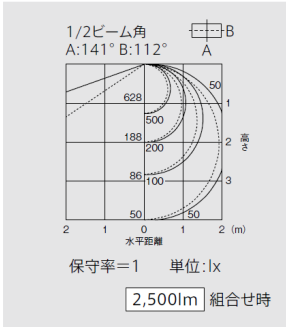
直付形2灯用業務用浴室灯 EL-LYWP4002
