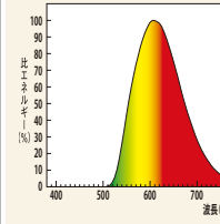
半導体工場向け LDL40T・Y/27/18・P-IC
