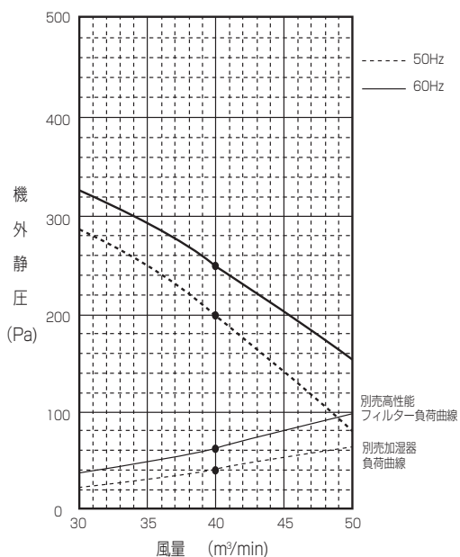
■PFFY-P140RM-G
