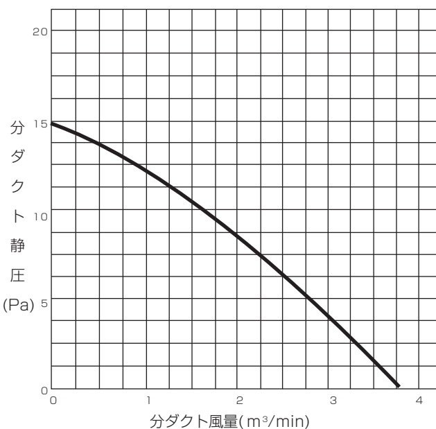
■PLFY-P140LM-G
