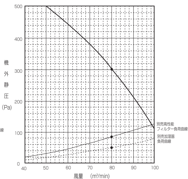
■PFFY-P280RM-G
