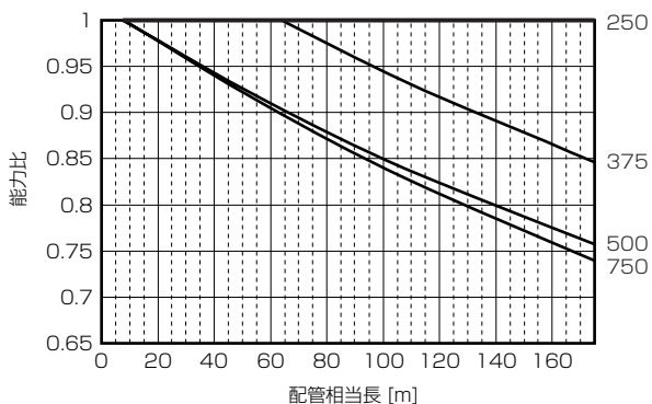
■PURY-P500SCM-G (-BS, -BSG)
