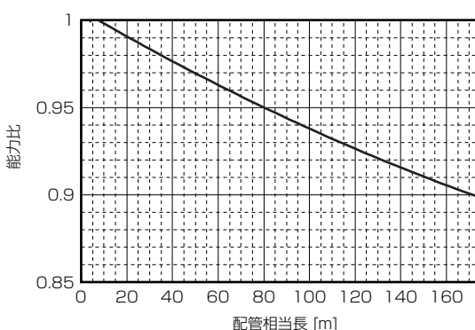
■PURY-P450, 500, 560(S) CM-G (-BS, -BSG)
