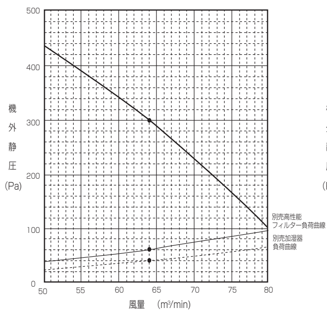
■PFFY-P224RM-G
