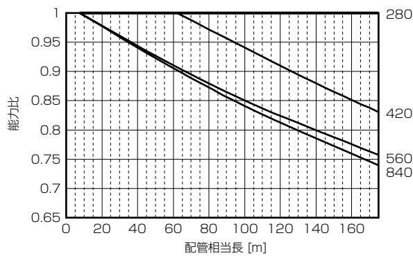
■PURY-P560SCM-G (-BS, -BSG)
