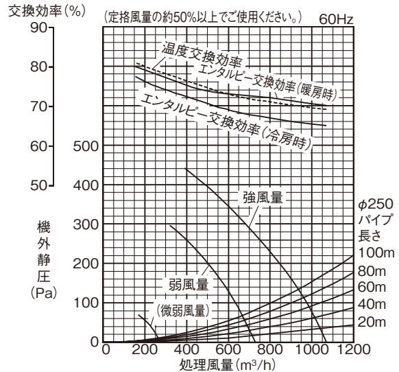
■ LGH-N80RDF 3 -60 (-DM)
