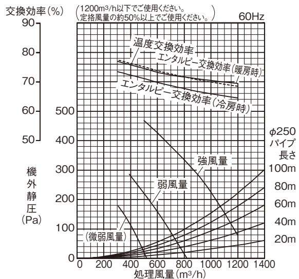
■ LGH-N100RDF 3 -60 (-DM)
