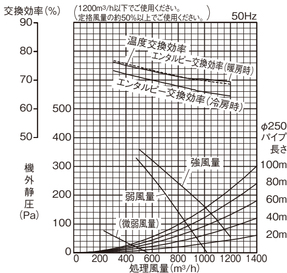
■ LGH-N100RDF 3 -50 (-DM)
