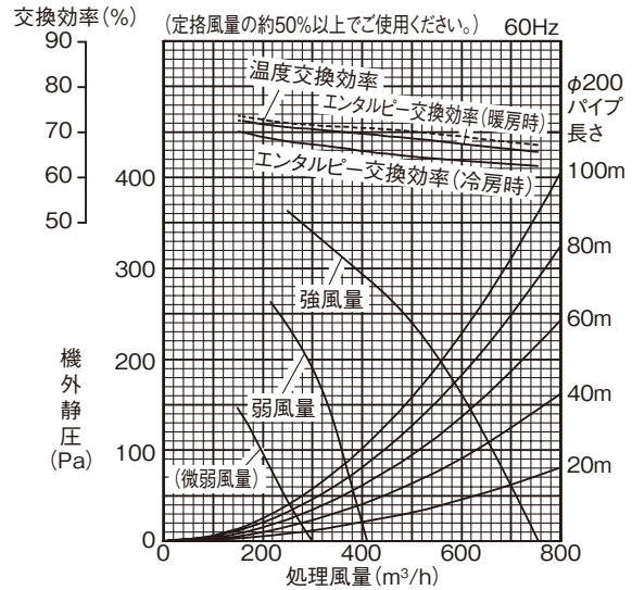
■ LGH-N50RDF 3 (-DM)
