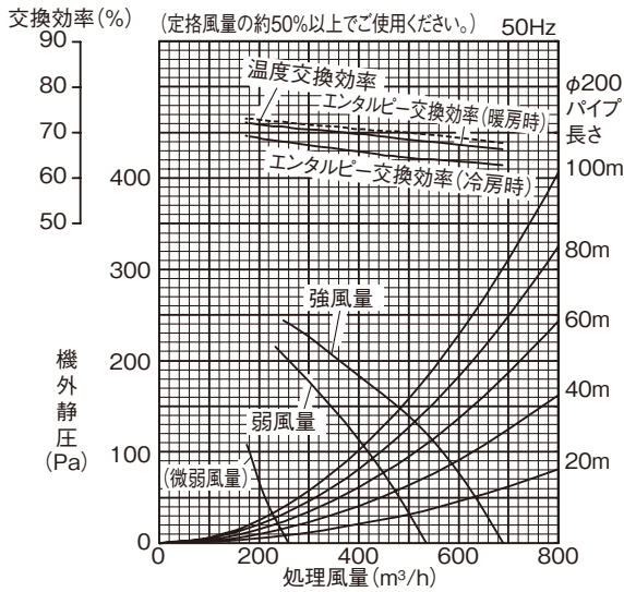
■ LGH-N50RDF 3 (-DM)
