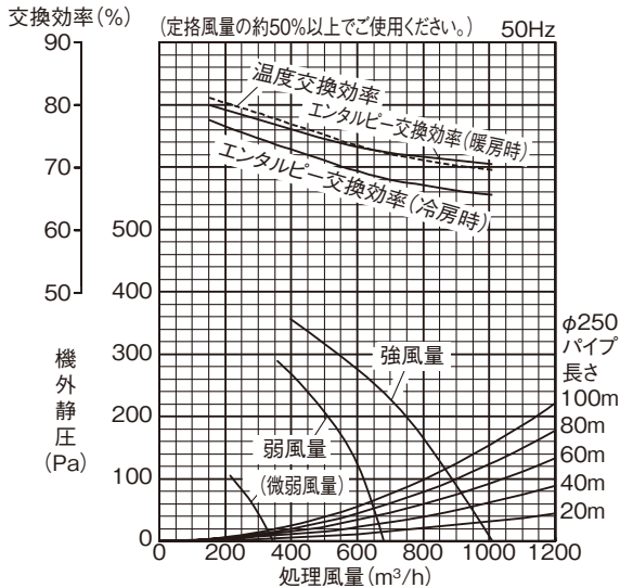
■ LGH-N80RDF 3 -50 (-DM)
