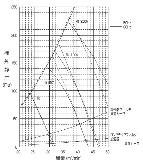
PE-RP160CA6
