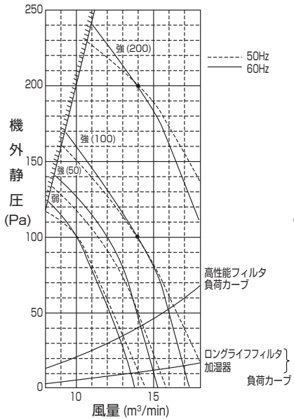
PE-RP112CA6, PE-RP140CA6
