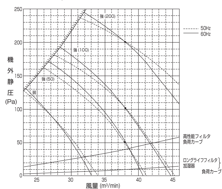
PE-RP112CA6, PE-RP140CA6
