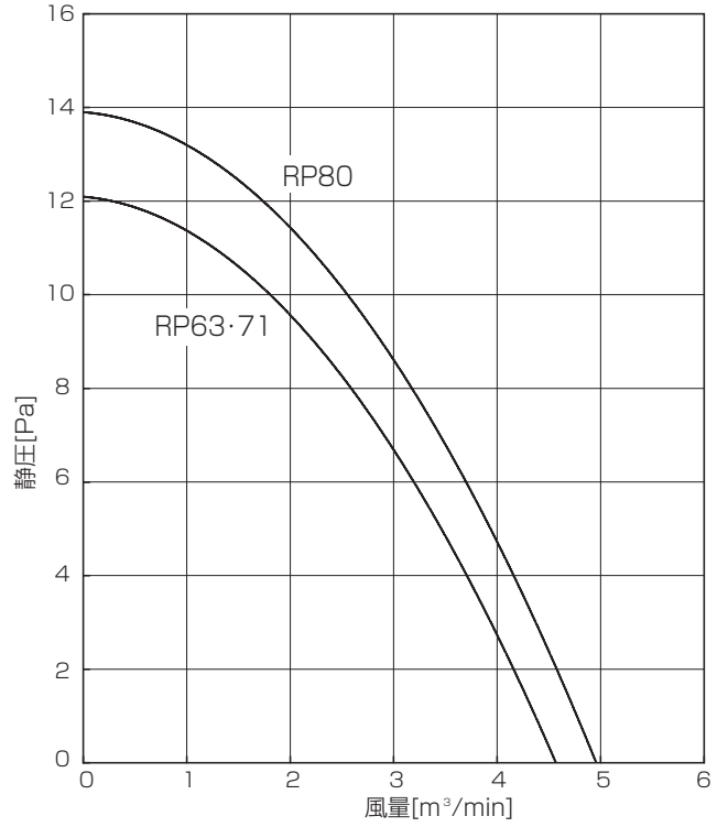
PL-RP71LA6, PL-RP80LA6
