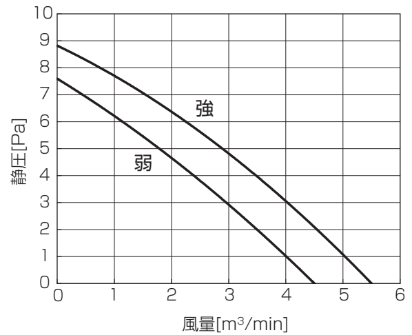
PS-RP71GA5, PS-RP80GA5
