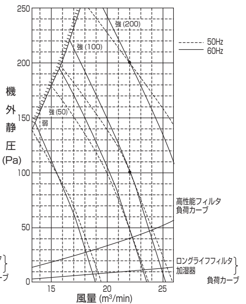
PE-RP160CA6
