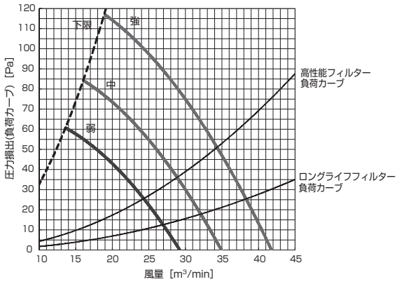
PD-RP140GA9 (機外静圧 70Pa)
