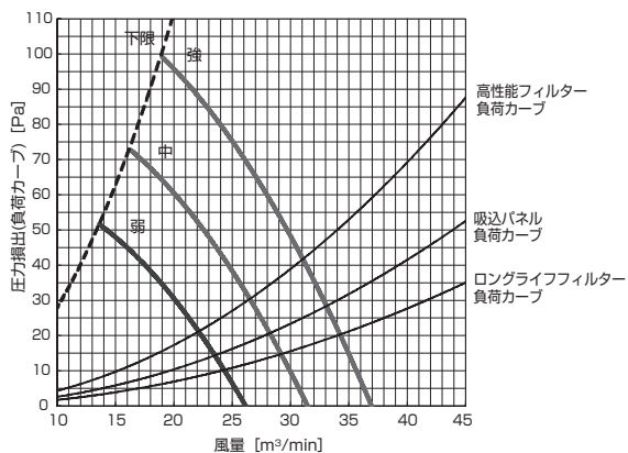
PD-RP112GA9 (機外静圧 20Pa)
