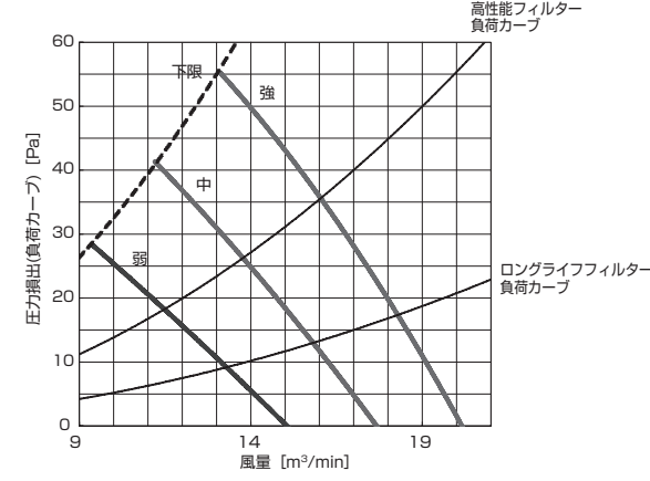
PD-RP40,56GA9 (機外静圧 130Pa)
