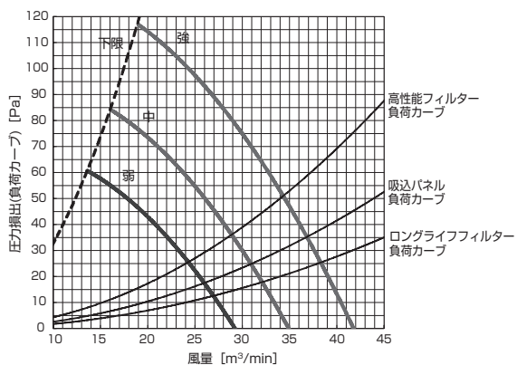
PD-RP140GA9 (機外静圧 70Pa)
