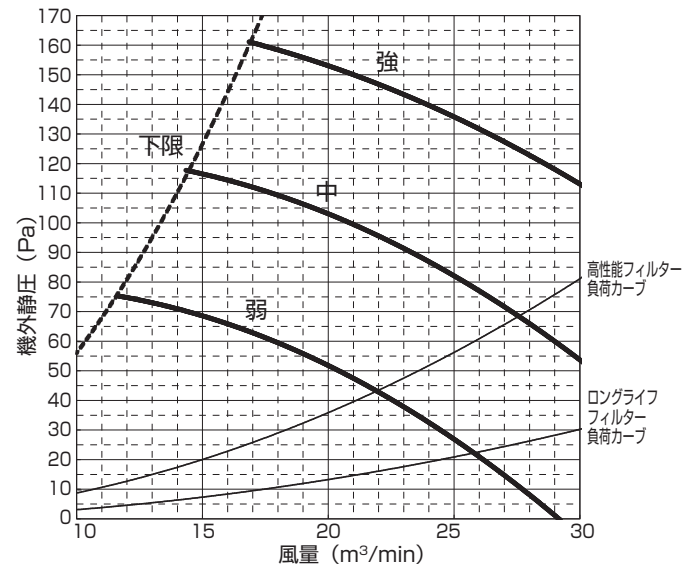
PE-RP71DA9 (機外静圧 150Pa)
