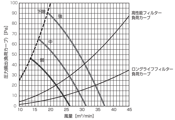
PD-RP140GA9 (機外静圧 120Pa)
