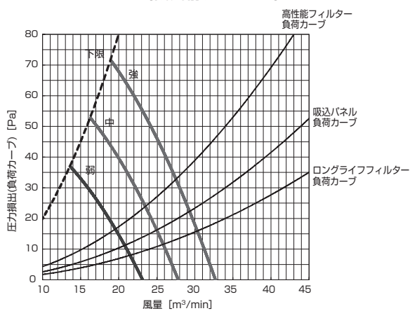
PD-RP112GA9 (機外静圧 110Pa)
