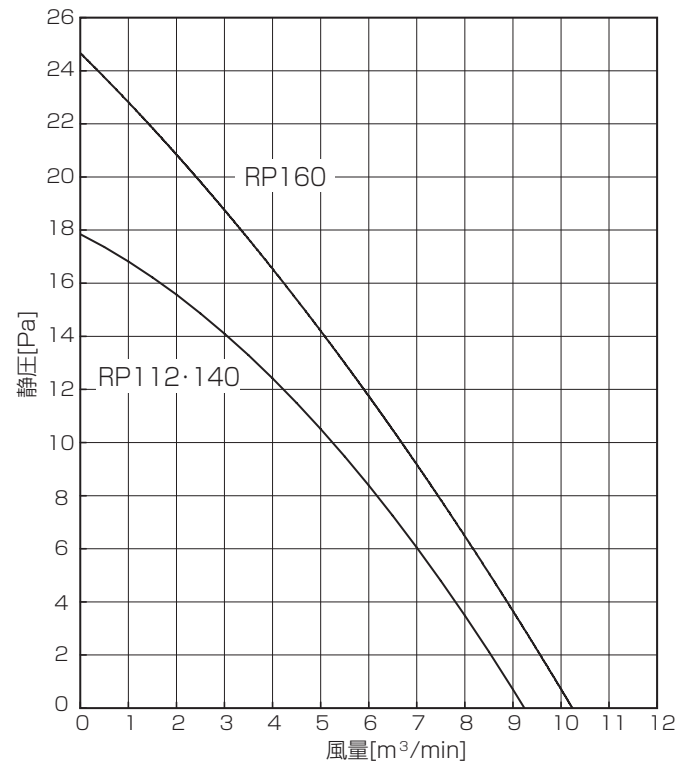
PL-RP112LA9, PL-RP140LA9, PL-RP160LA9
