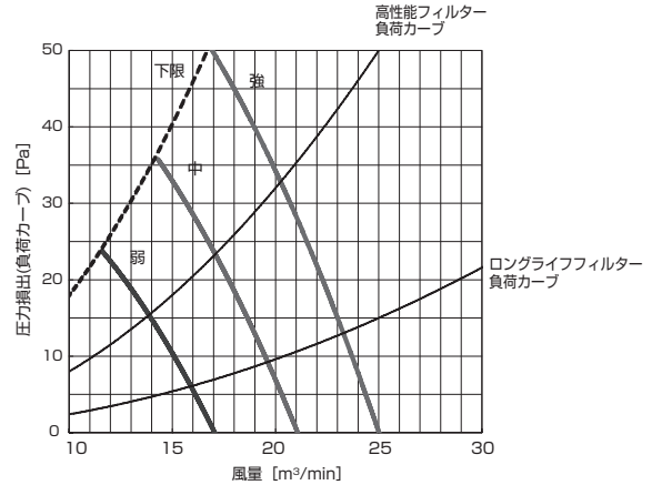
PD-RP71,80GA9 (機外静圧 120Pa)
