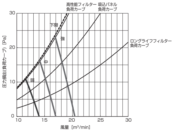
PD-RP71,80GA9 (機外静圧 60Pa)
