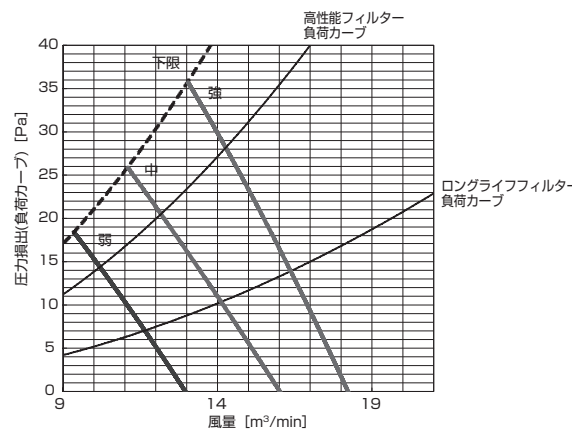
PD-RP40,56GA9 (機外静圧 80Pa)
