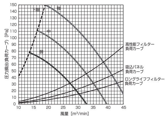
PD-RP112GA9 (機外静圧 120Pa)
