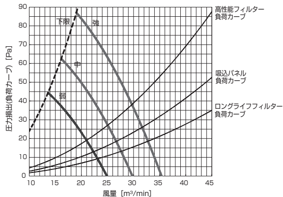
PD-RP140GA9 (機外静圧 110Pa)
