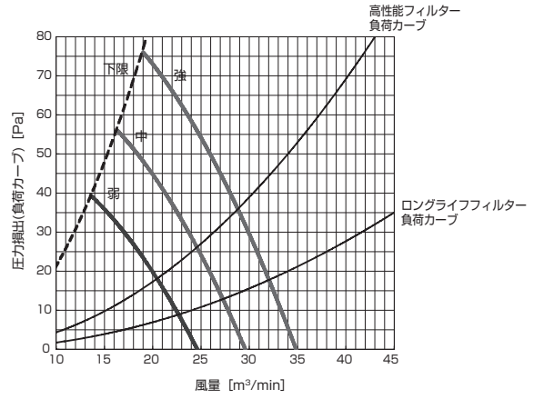
PD-RP112GA9 (機外静圧 120Pa)
