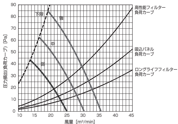
PD-RP160GA9 (機外静圧 60Pa)
