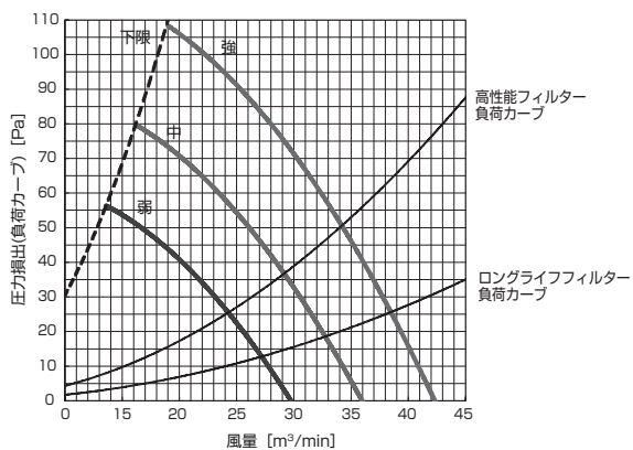
PD-RP112GA9 (機外静圧 80Pa)
