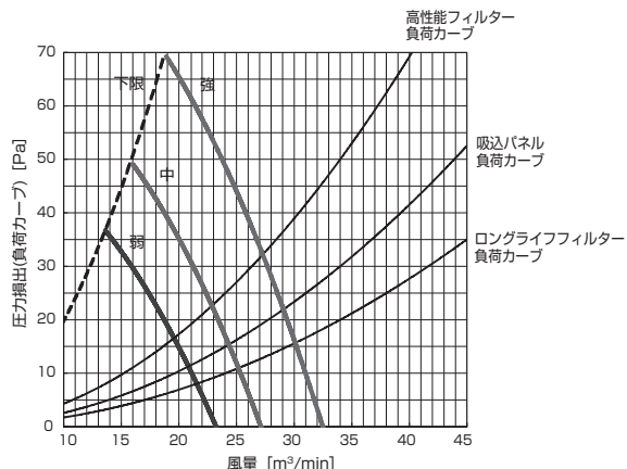
PD-RP140GA9 (機外静圧 60Pa)
