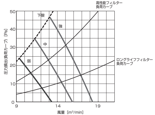
PD-RP40,56GA9 (機外静圧 120Pa)
