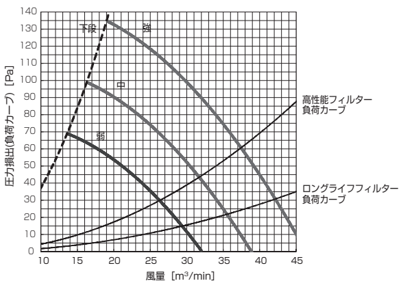
PD-RP160GA9 (機外静圧 80Pa)
