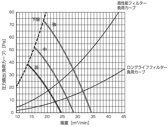
PD-RP140GA9 (機外静圧 70Pa)
