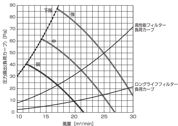
PD-RP71,80GA9 (機外静圧 80Pa)
