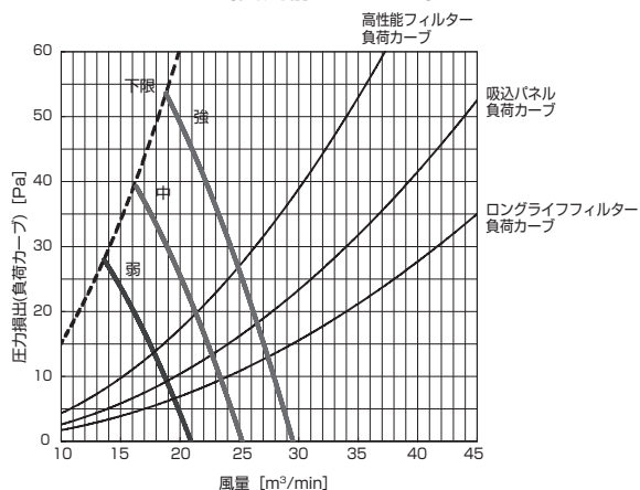
PD-RP112GA9 (機外静圧 60Pa)
