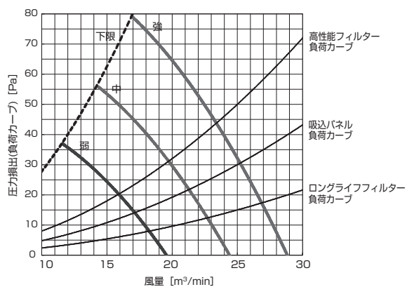
PD-RP71,80GA9 (機外静圧 70Pa)
