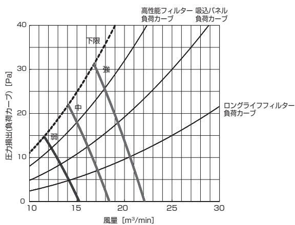
PD-RP71,80GA9 (機外静圧 70Pa)
