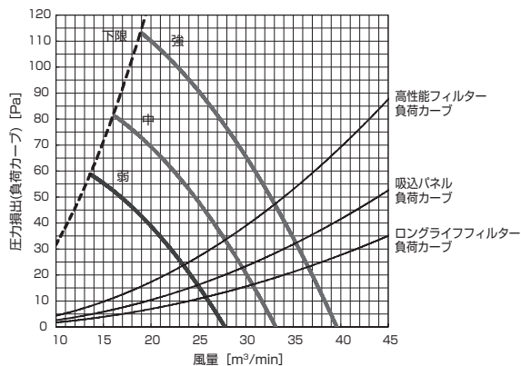
PD-RP140GA9 (機外静圧 20Pa)
