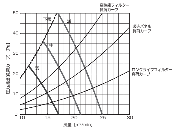
PD-RP71,80GA9 (機外静圧 120Pa)
