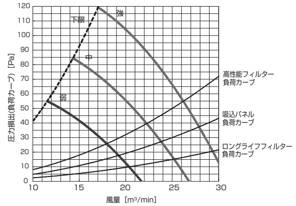
PD-RP71,80GA9 (機外静圧 110Pa)
