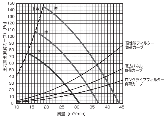
PD-RP112GA9 (機外静圧 40Pa)
