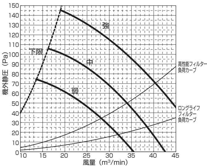
PE-RP112DA9 (機外静压 100Pa)
