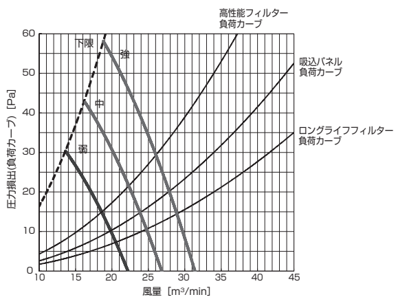
PD-RP112GA9 (機外静圧 70Pa)
