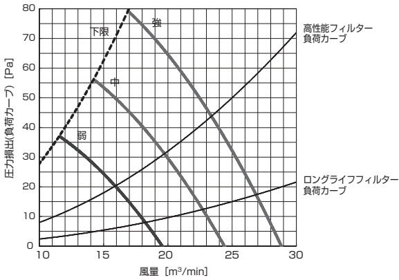
PD-RP71,80GA9 (機外静圧 70Pa)
