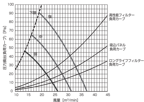
PD-RP140GA9 (機外静圧 120Pa)
