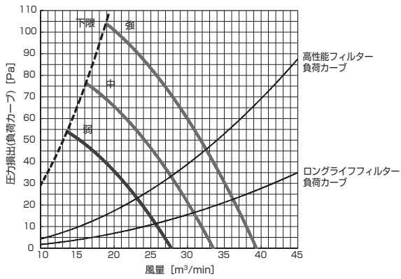
PD-RP112GA9 (機外静圧 70Pa)
