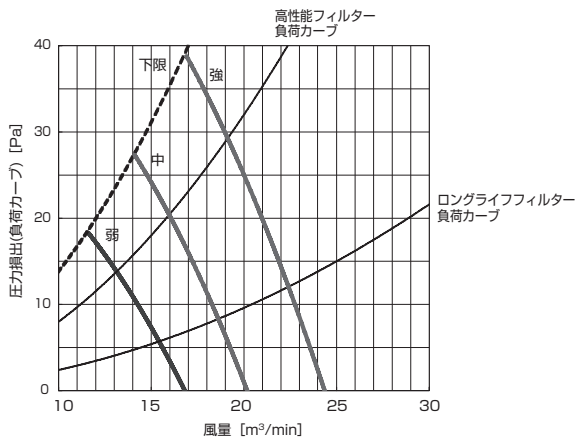
PD-RP71,80GA9 (機外静圧 80Pa)
