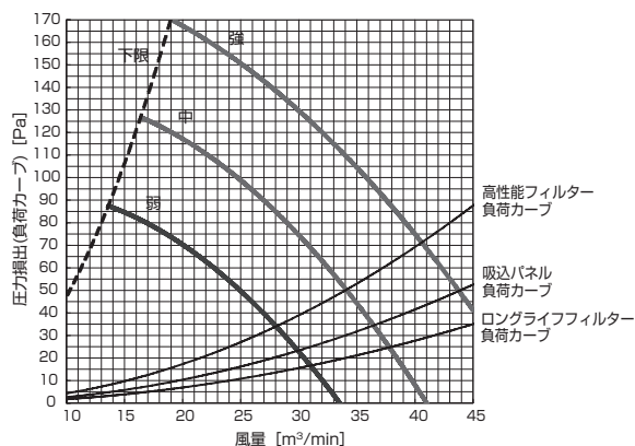
PD-RP160GA9 (機外静圧 110Pa)
