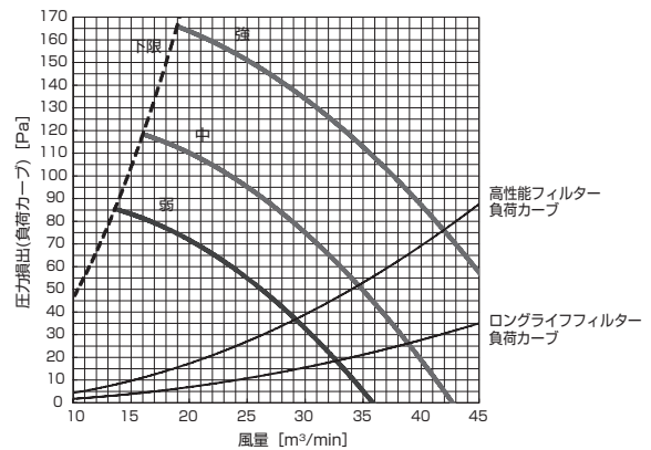
PD-RP140GA9 (機外静圧 130Pa)
