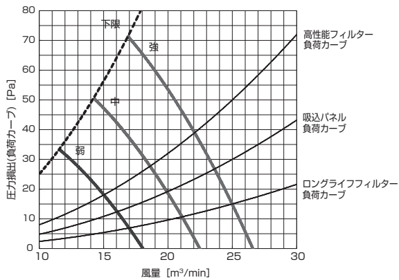
PD-RP71,80GA9 (機外静圧 60Pa)
