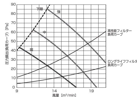
PD-RP40,56GA9 (機外静圧 80Pa)
