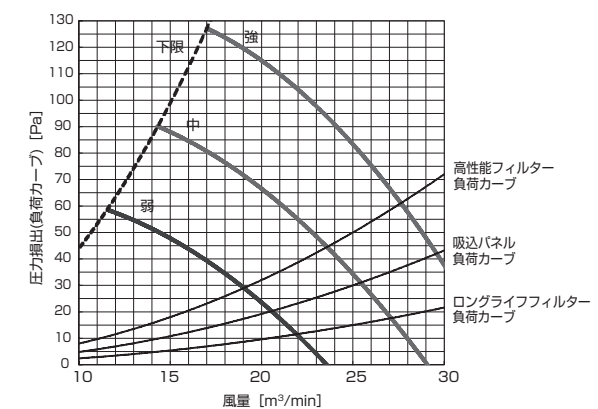
PD-RP71,80GA9 (機外静圧 120Pa)
