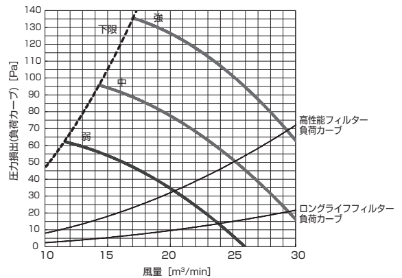
PD-RP71,80GA9 (機外静圧 130Pa)
