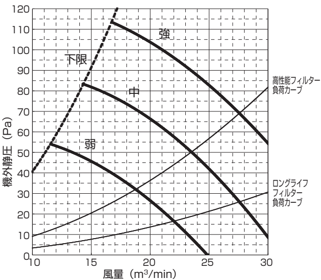
PE-RP71DA9 (機外静圧 100Pa)
