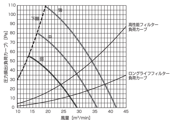
PD-RP160GA10 (機外静圧 130Pa)
