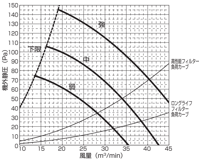
PE-RP112DA10(機外静圧 100Pa)
