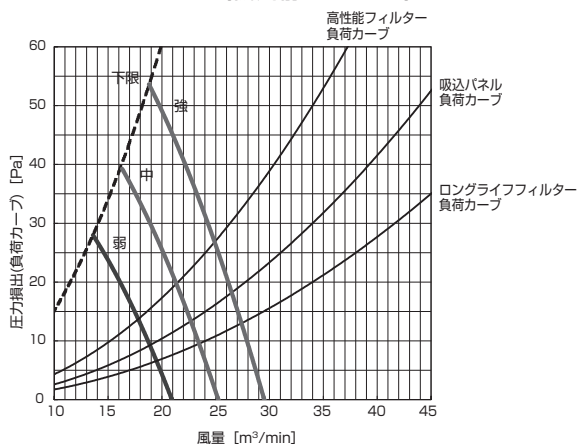
PD-RP112GA10 (機外静圧 60Pa)
