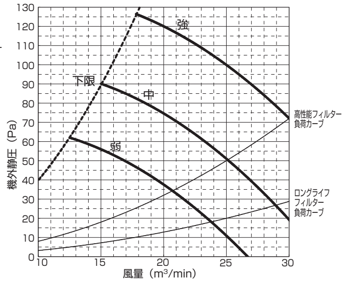
PE-RP112DA10(機外静圧 50Pa)
