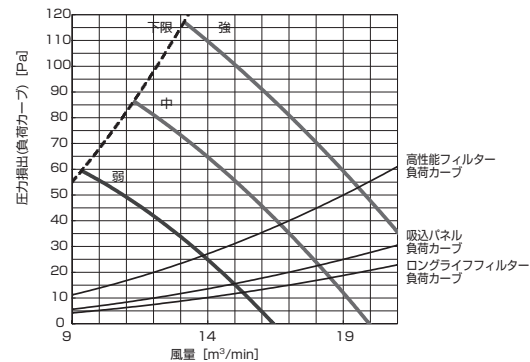
PD-RP40,50,56GA10 (機外静圧 110Pa)
