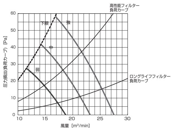
PD-RP63,71,80GA10 (機外静圧 130Pa)
