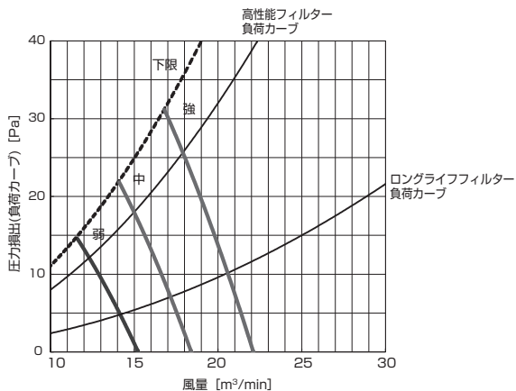
PD-RP63,71,80GA10 (機外静圧 70Pa)
