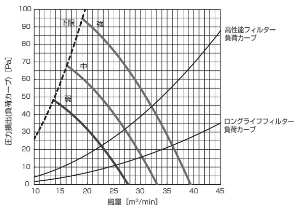
PD-RP140GA10 (機外静圧 130Pa)
