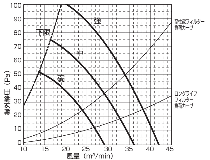
PE-RP112DA10(機外静圧 50Pa)
