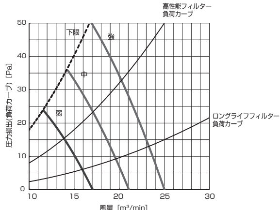
PD-RP63,71,80GA10 (機外静圧 120Pa)
