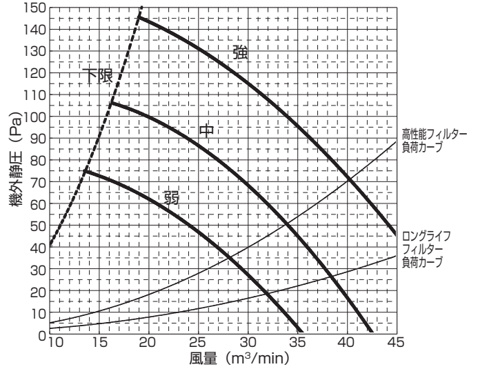
PE-RP140DA10(機外静压 100Pa)
