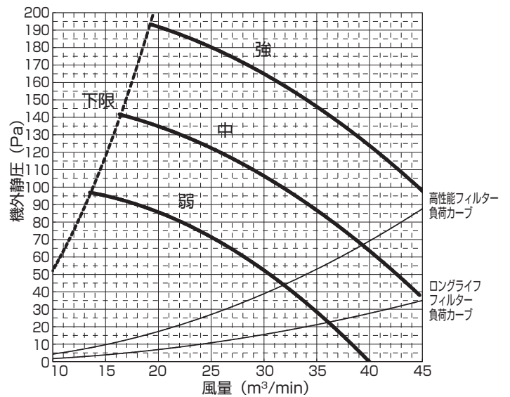
PE-RP112DA10(機外静圧 150Pa)
