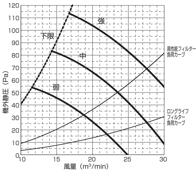
PE-RP71DA10(機外静压 100Pa)
