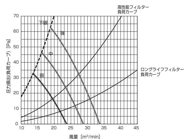
PD-RP112GA10 (機外静圧 80Pa)
