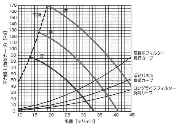
PD-RP160GA10 (機外静圧 40Pa)
