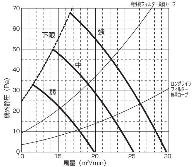
PE-RP71DA10(機外静压 50Pa)
