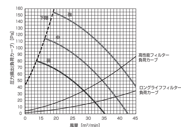
PD-RP112GA10 (機外静圧 130Pa)
