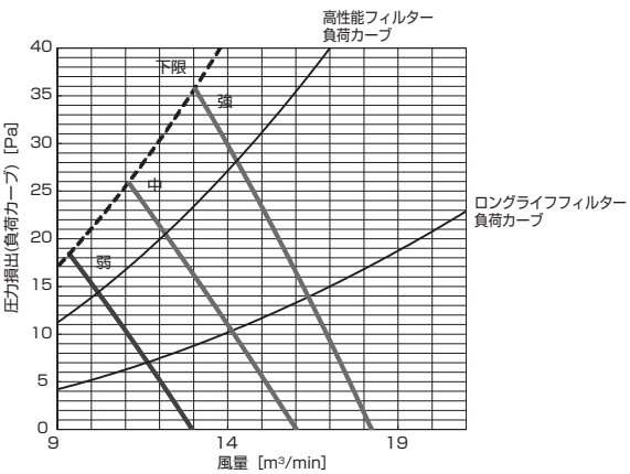
PD-RP40,50,56GA10 (機外静圧 80Pa)
