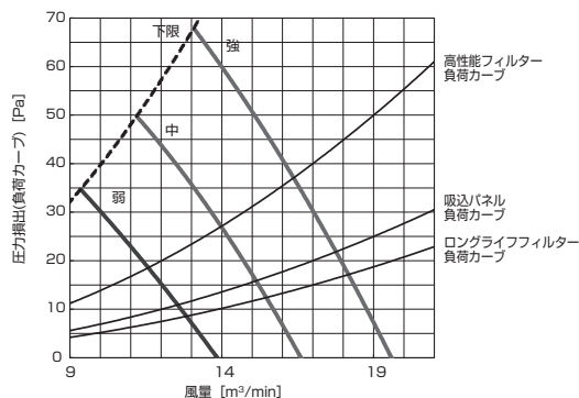
PD-RP40,50,56GA10 (機外静圧 60Pa)
