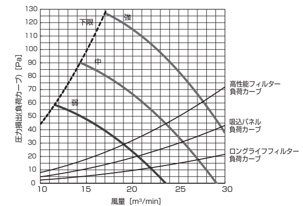
PD-RP63,71,80GA10 (機外静圧 120Pa)
