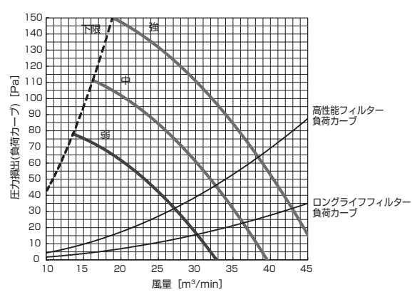
PD-RP112GA10 (機外静圧 120Pa)
