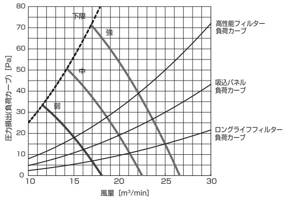
PD-RP63,71,80GA10 (機外静圧 60Pa)
