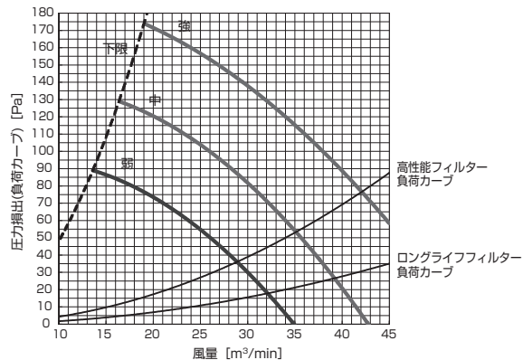
PD-RP160GA10 (機外静圧 120Pa)
