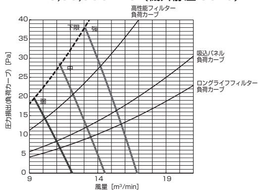
PD-RP40,50,56GA10 (機外静圧 110Pa)
