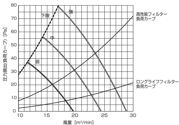
PD-RP63,71,80GA10 (機外静圧 70Pa)
