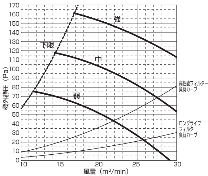
PE-RP63DA10(機外静压 150Pa)
