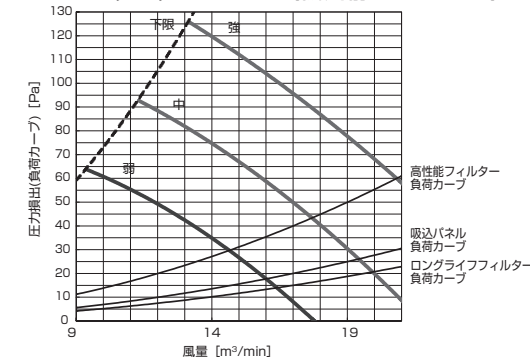
PD-RP40,50,56GA10 (機外静圧 120Pa)
