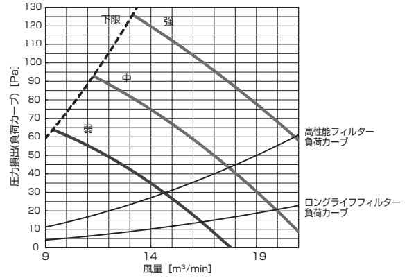
PD-RP40,50,56GA10 (機外静圧 50Pa)
