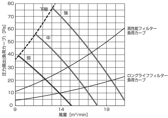
PD-RP40,50,56GA10 (機外静圧 30Pa)
