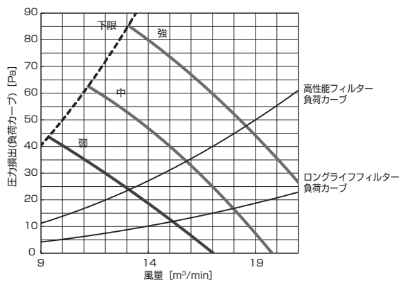
PD-RP40,50,56GA10 (機外静圧 80Pa)
