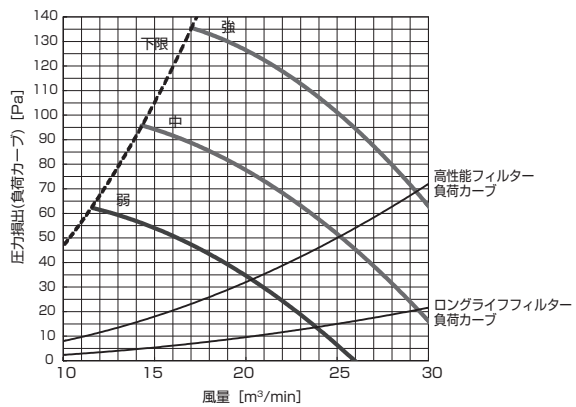
PD-RP63,71,80GA10 (機外静圧 130Pa)
