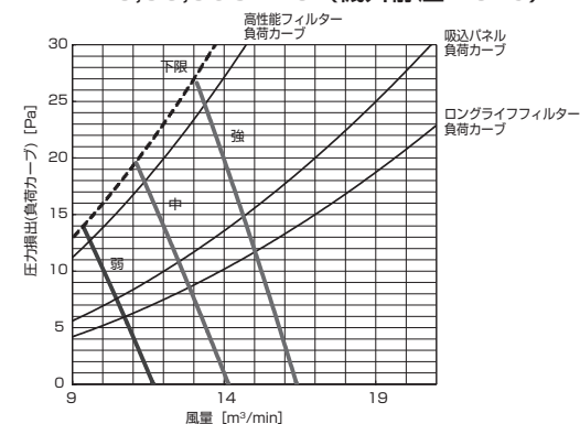
PD-RP40,50,56GA10 (機外静圧 70Pa)
