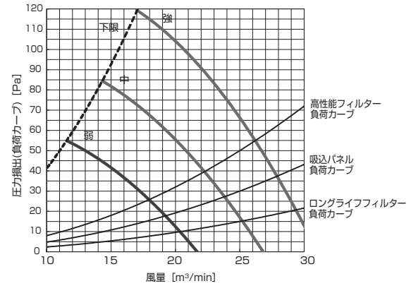
PD-RP63,71,80GA10 (機外静圧 110Pa)
