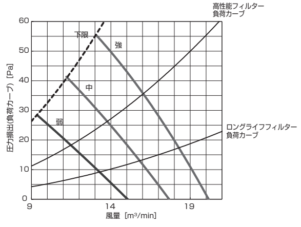
PD-RP40,50,56GA10 (機外静圧 130Pa)
