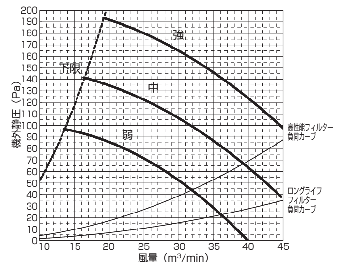
PE-RP160DA10(機外静压 150Pa)
