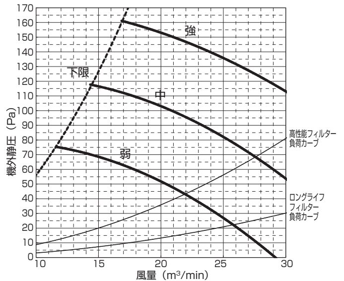
PE-RP71DA10(機外静压 150Pa)
