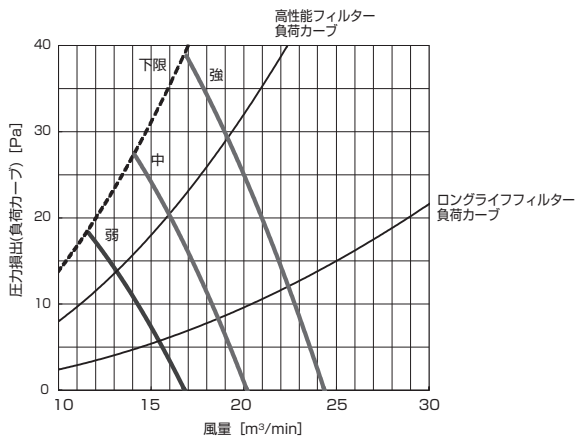
PD-RP63,71,80GA10 (機外静圧 80Pa)
