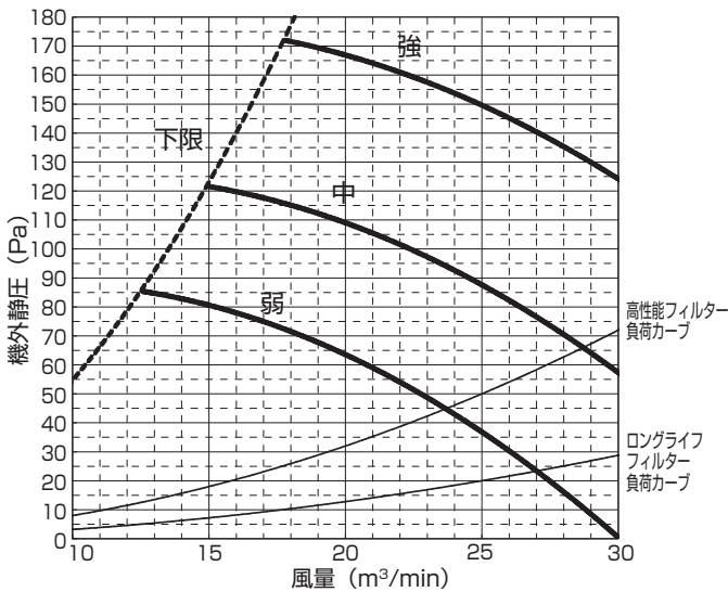
PE-RP80DA10(機外静圧 150Pa)
