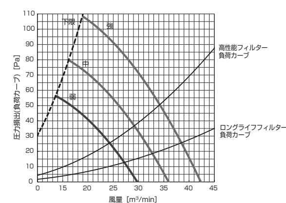
PD-RP112GA10 (機外静圧 80Pa)
