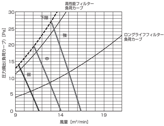
PD-RP40,50,56GA10 (機外静圧 70Pa)
