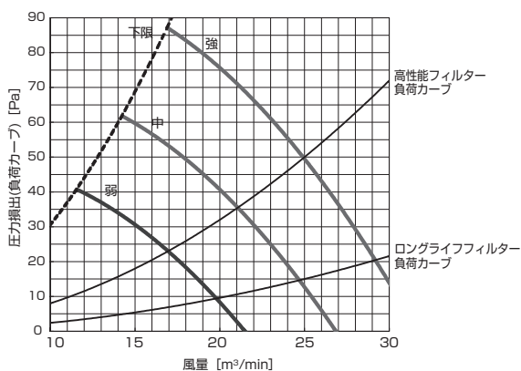
PD-RP63,71,80GA10 (機外静圧 80Pa)
