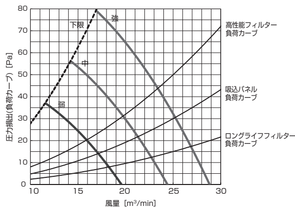
PD-RP63,71,80GA10 (機外静圧 70Pa)
