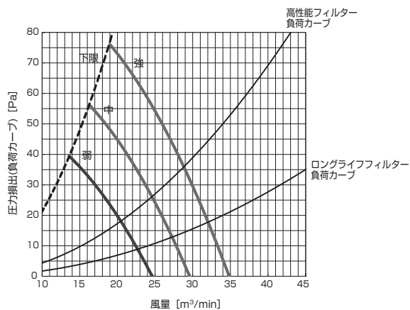
PD-RP112GA10 (機外静圧 120Pa)
