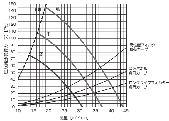
PD-RP112GA10 (機外静圧 40Pa)
