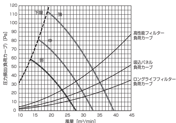
PD-RP140GA10 (機外静圧 60Pa)
