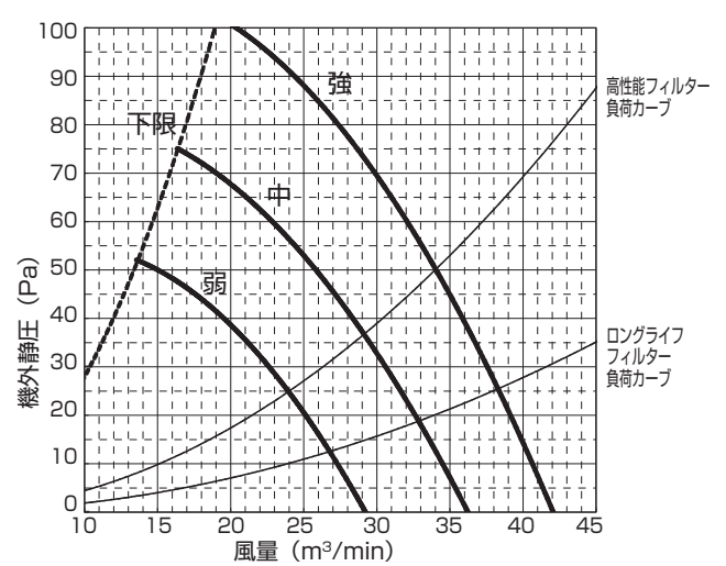
PE-RP160DA10(機外静压 50Pa)
