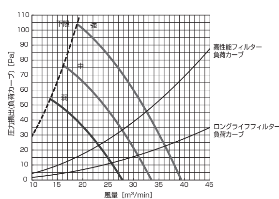
PD-RP112GA10 (機外静圧 70Pa)
