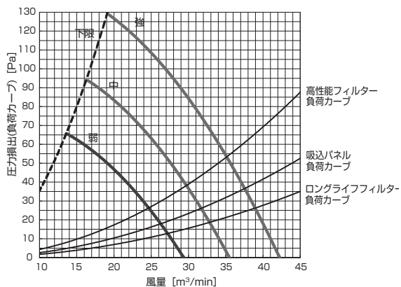
PD-RP160GA10 (機外静圧 20Pa)
