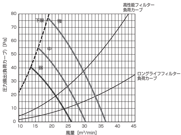
PD-RP140GA10 (機外静圧 80Pa)
