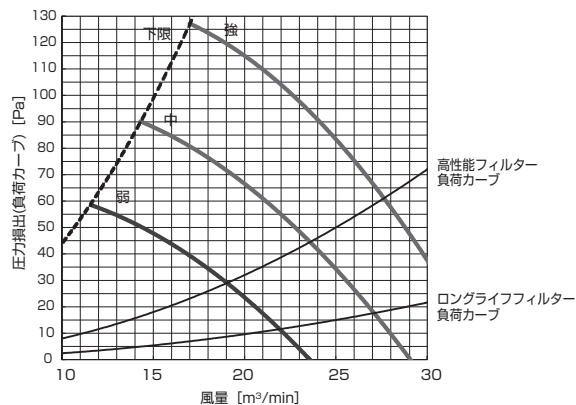
PD-RP63,71,80GA10 (機外静圧 120Pa)
