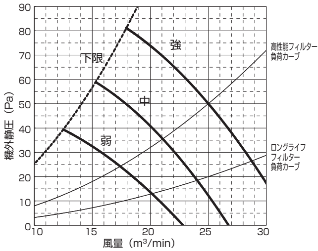
PE-RP80DA10(機外静圧 50Pa)
