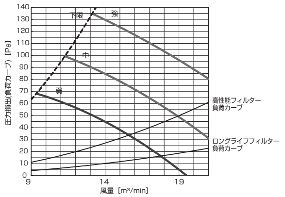
PD-RP40,50,56GA10 (機外静圧 130Pa)
