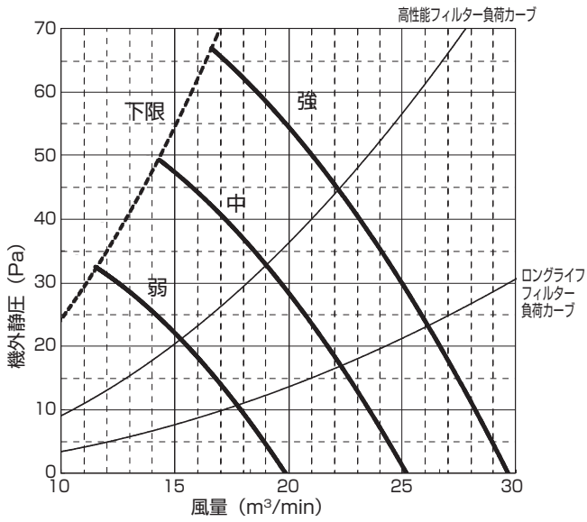
PE-RP63DA10(機外静压 50Pa)
