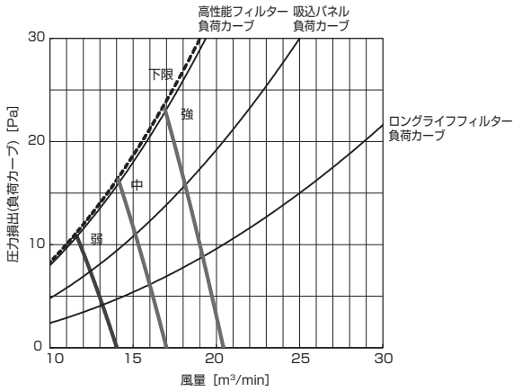
PD-RP63,71,80GA10 (機外静圧 60Pa)
