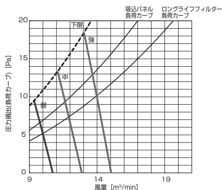
PD-RP40,50,56GA10 (機外静圧 60Pa)
