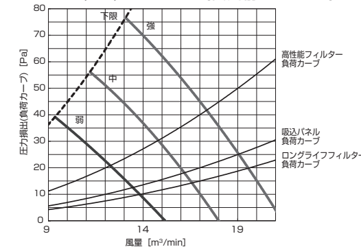
PD-RP40,50,56GA10 (機外静圧 70Pa)
