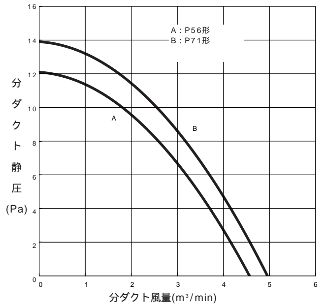
PLFY-P56・P71LMD-E1
