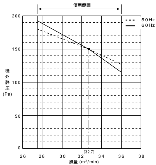
PFFY-P280RM-E1-F
