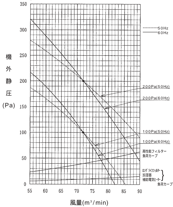
PEFY-P280M-E1
