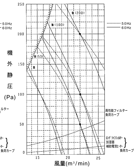
PEFY-P80M-E1
