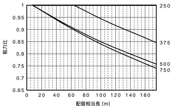
PURY-P500SCM-E(-BS, -BSG)
