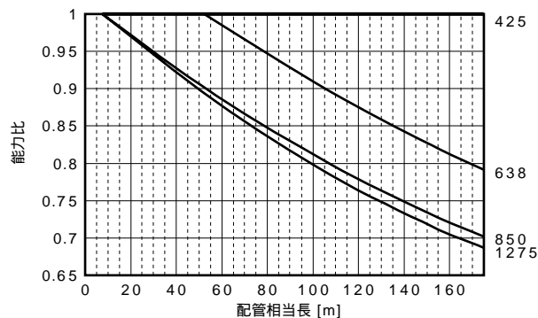
PURY-P850SCM-E(-BS, -BSG)
