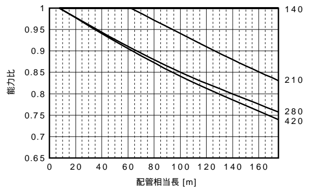
PURY-P280CM-E(-BS, -BSG)
