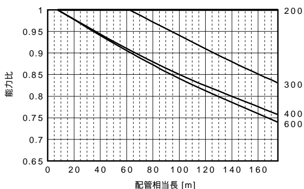
PURY-P400CM-E(-BS, -BSG)
