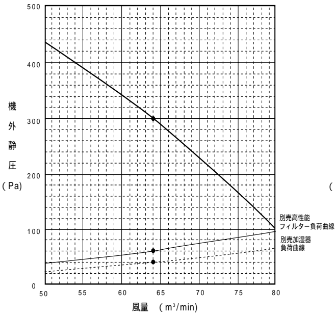
PFFY-P224RM-E1
