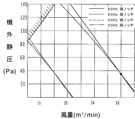
PDFY-P112M-E1
