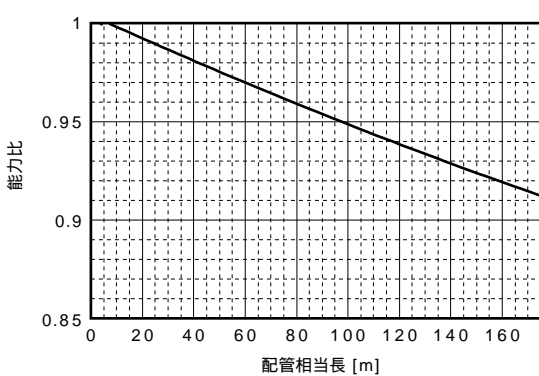
PURY-P224CM-E(-BS, -BSG)
