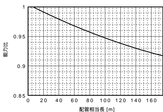
PURY-P400CM-E(-BS, -BSG)
