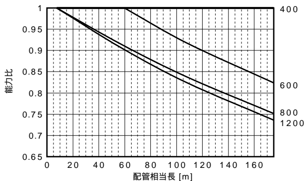
PURY-P800SCM-E(-BS, -BSG)
