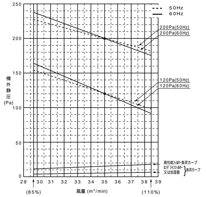
PEFY-P280M-E1-F
