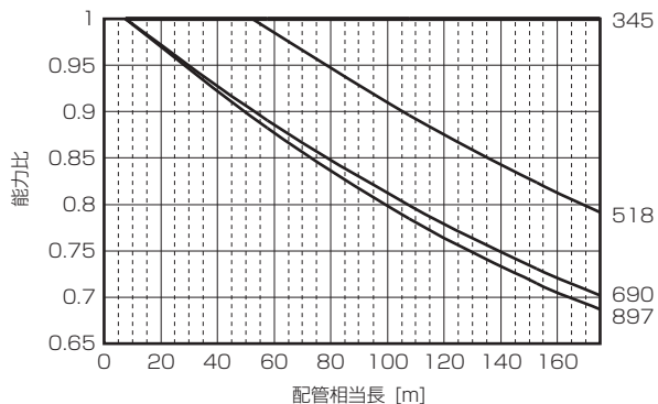
■PUHY-EP800SDMG2
