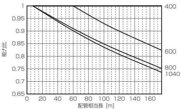
■PUHY-EP800SDMG2
