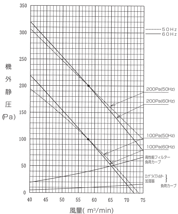
■PEFY-P224MG1
