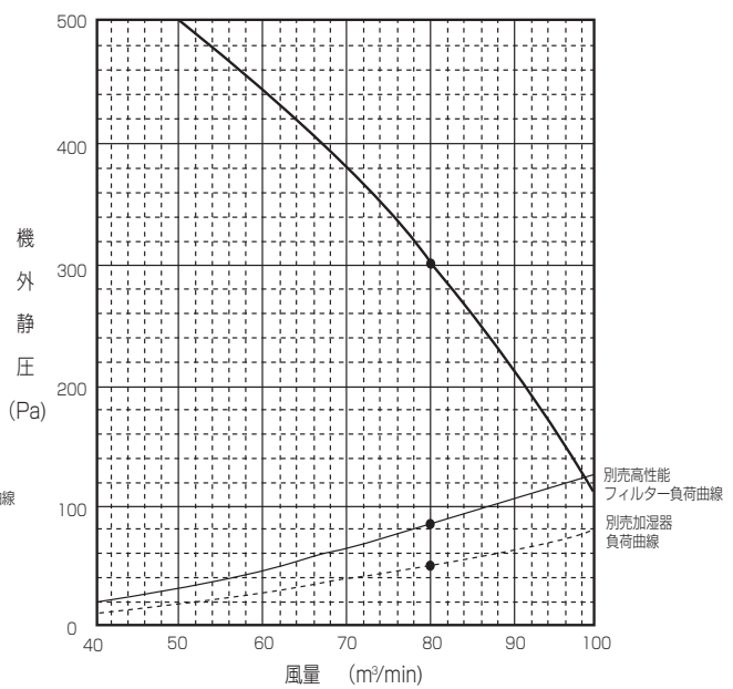
■PFFY-P280RMG1
