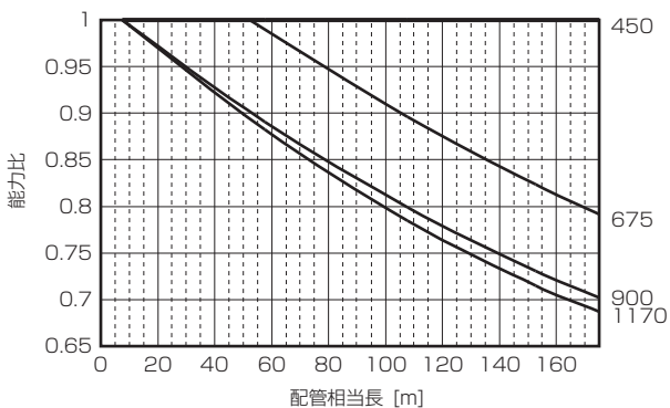
■PUHY-EP900SDMG2
