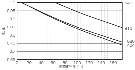
■PUHY-EP1180SDMG2
