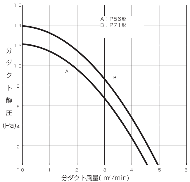
■PLFY-P56・P71LMG1
