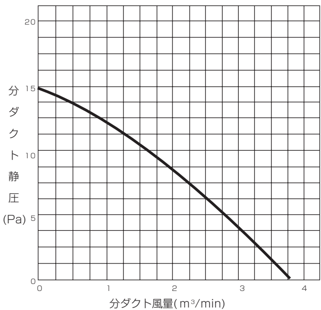
■PLFY-P140LMG1
