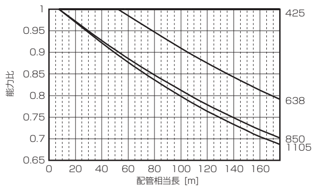
■PUHY-EP850SDMG2
