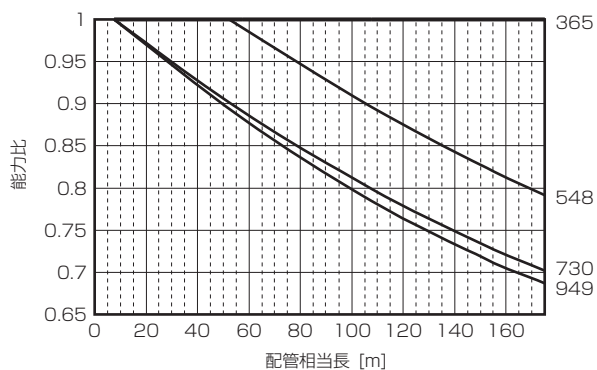
■PUHY-EP730SDMG2
