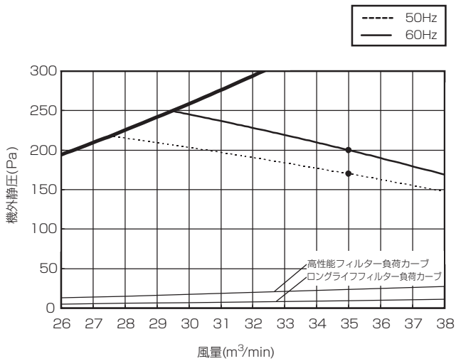
■GE-P2100MG1
