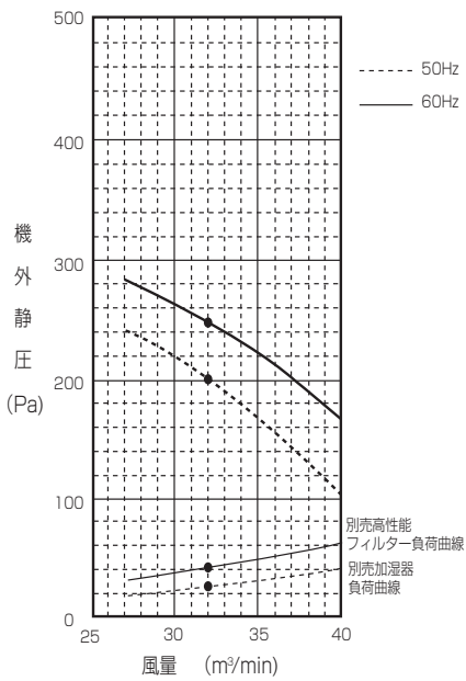
■PFFY-P112RMG1
