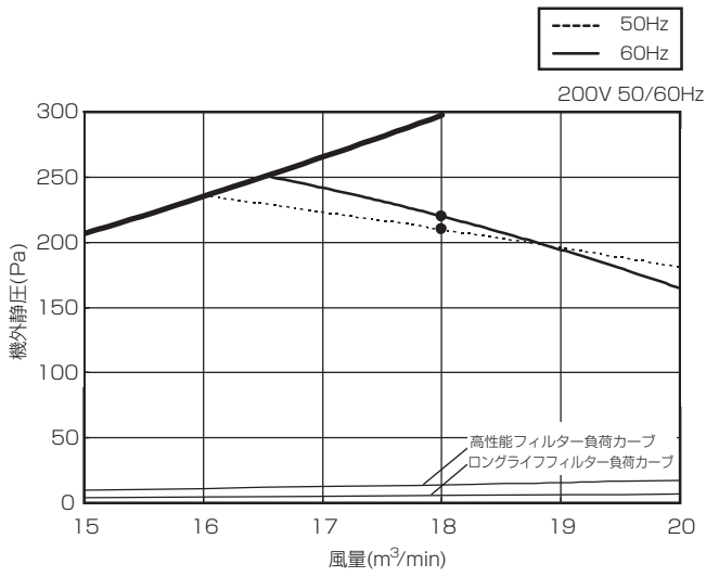
■GE-P1080MG1
