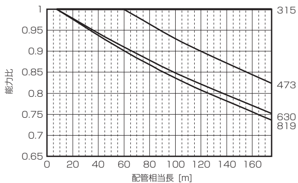
■PUHY-EP730SDMG2
