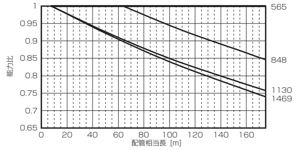
■PUHY-EP1240SDMG2
