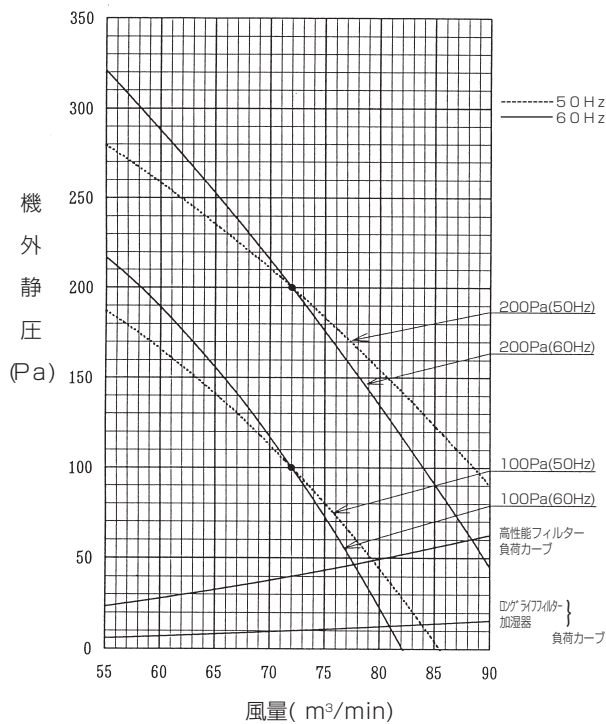
■PEFY-P280MG1
