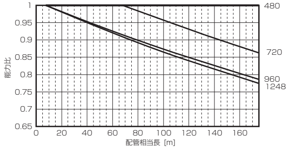
■PUHY-EP1080SDMG2
