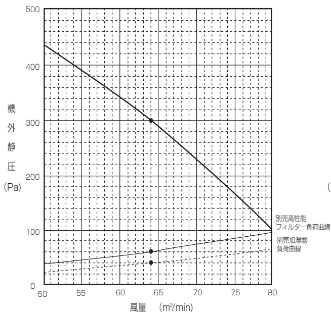
■PFFY-P224RMG1
