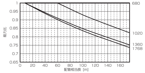
■PUHY-EP1360SDMG2
