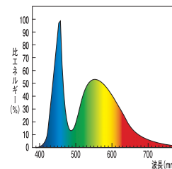
LDA11D-H/D(昼光色)
