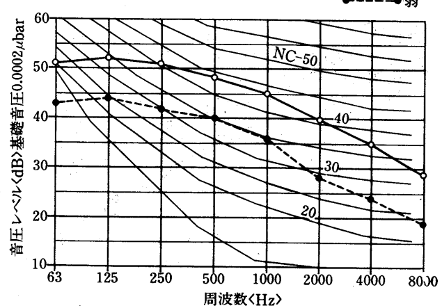
PSH-100AD形
