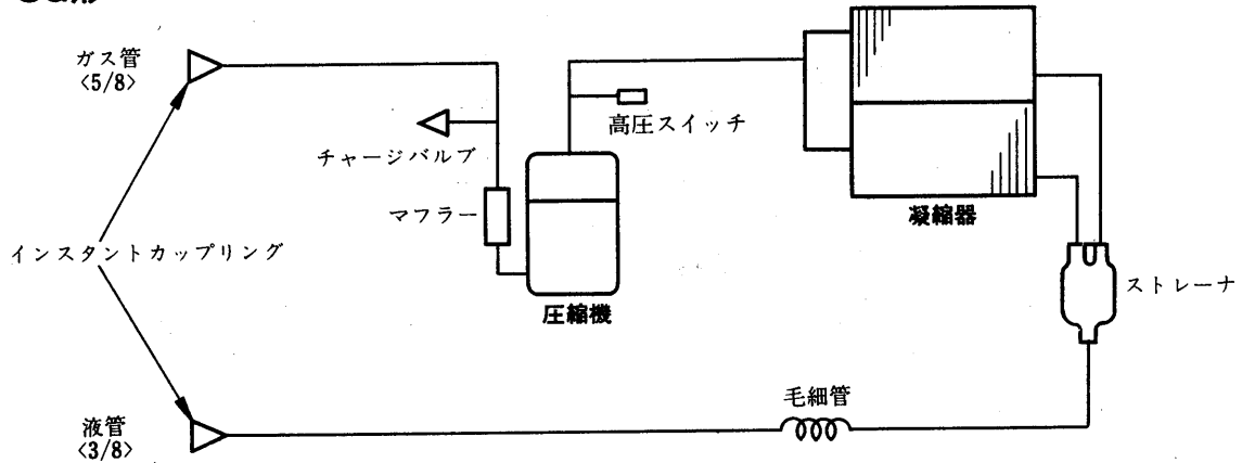
(M)PU-100G形
