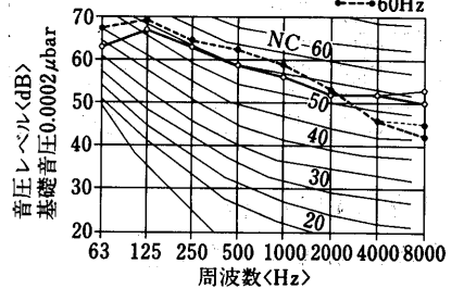
PUTF-15A形
