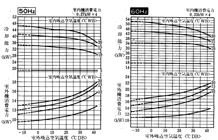
PCTF-J375PMB形<PUTF-J375A/PCT-J95PA×4>
