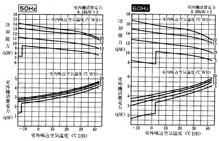
PCTF-J125PMB形<PUTF-J125B/PCT-J71PA×2>
