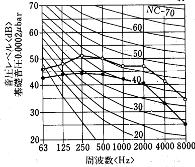
PUTF-J250B形
