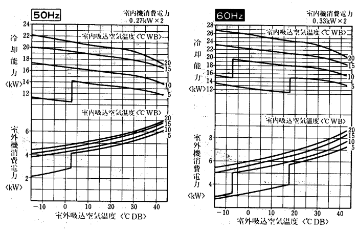
PCTF-J190PMB形<PUTF-J190B/PCT-J95PA×2>
