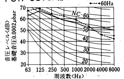
PUTF-J375A形
