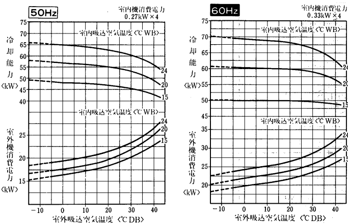
PCTF-J560PHB形<PUTF-J500A/PCT-J95PA×4>
