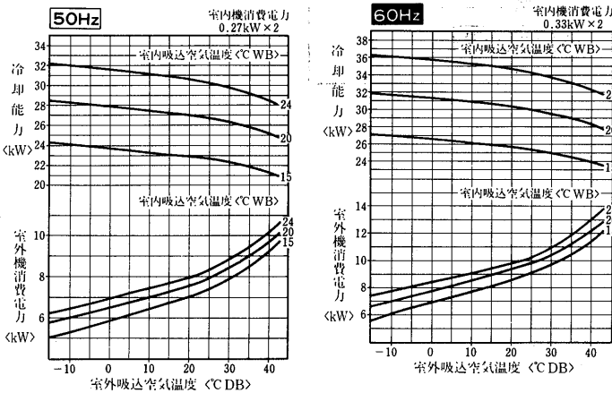
PCTF-J280PHB形<PUTF-J250B/PCT-J95PA×2>
