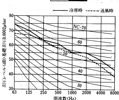
PAT-J670G形 [50Hz]
