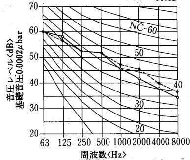
PUTF-J500A形
