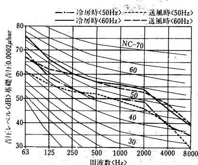
PAT-J530G形 [50Hz]
