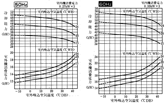
PCTF-J425PHB形<PUTF-J375A/PCT-J95PA×3>
