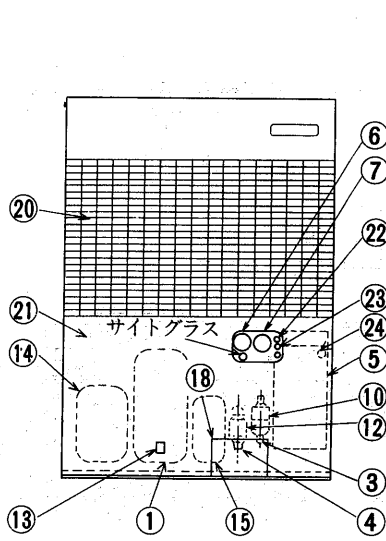
PUTF-J375A形
