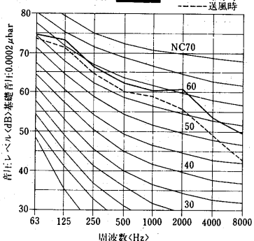
PAT-J670G形 [60Hz]
