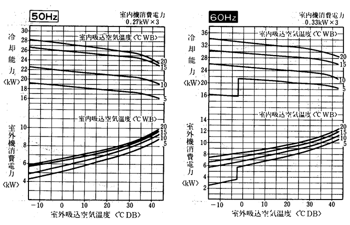
PCTF-J265PMB形<PUTF-J250B/PCT-J95PA×3>
