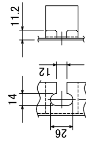
C (吊りボルト用穴詳細図)
