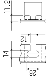
A (吊りボルト用穴詳細図)
