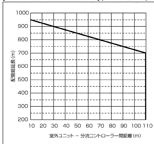
【PURY-P800/850/900SCM-E】(28/30/32HP)
