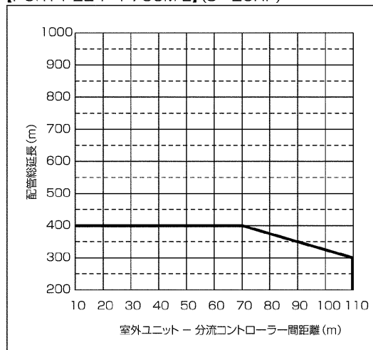
【PURY-P224~P730M-E】(8~26HP)
