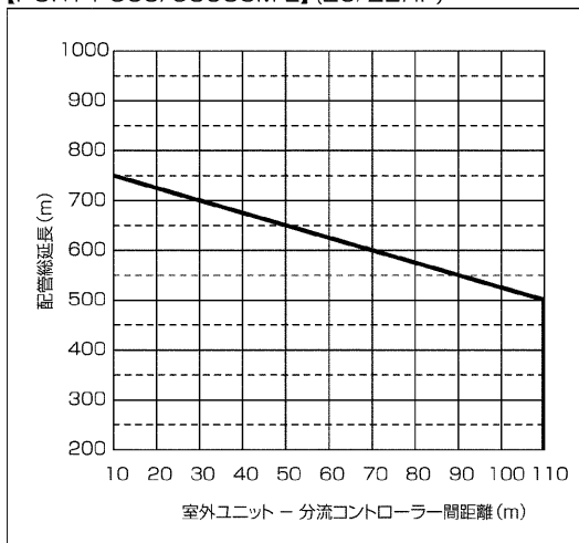
【PURY-P560/630SCM-E】(20/22HP)
