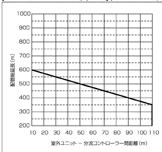
【PURY-P400/450/500(S)CM-E】(14/16/18HP)
