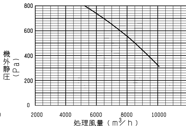
LP-1000X 2
