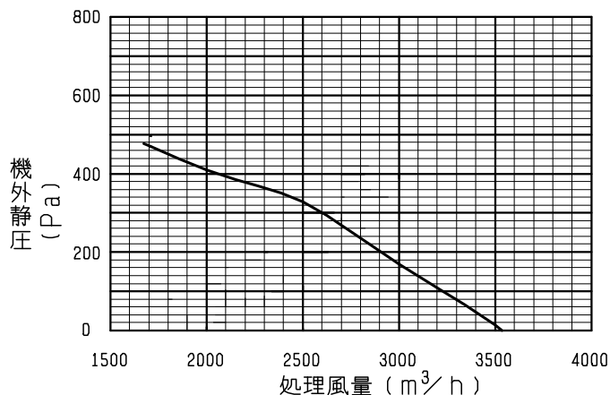
LP-250X 2
