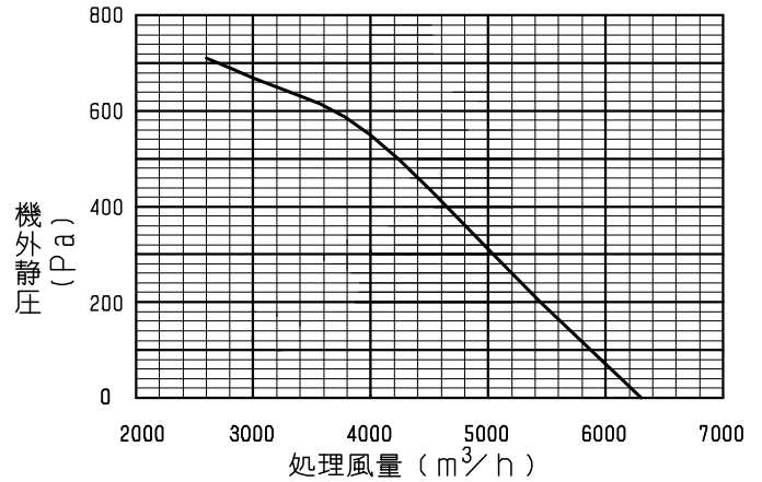
LP-500X 3 , X 4
