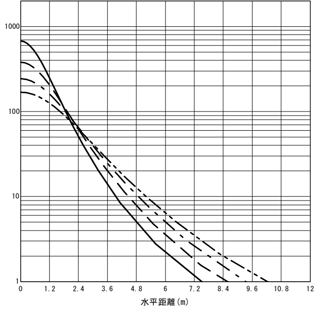
○直射水平面照度 (全光束: 5000 × 1 = 5000lm/台) 照度 (lx) — H1.50m --- H2.00m - - - H2.50m ····· H3.00m (保守率: 1.00)
