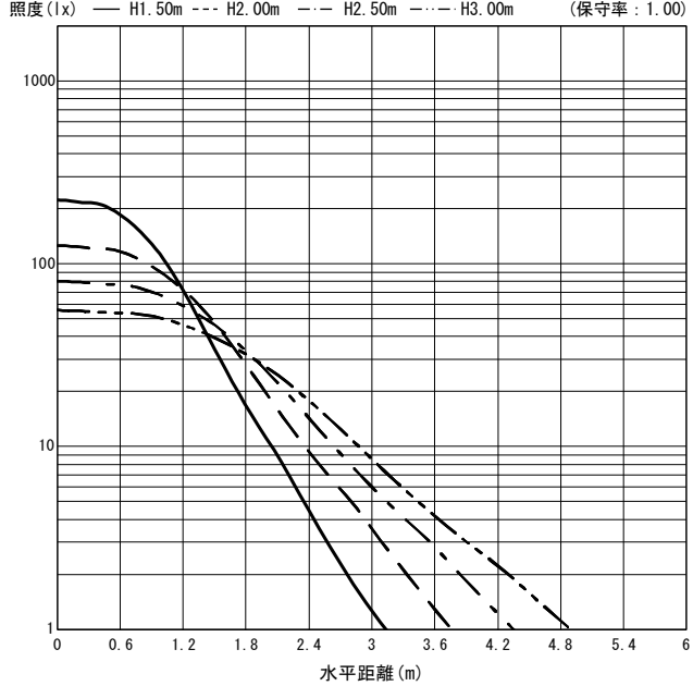
○直射水平面照度 (全光束 : 970 × 1 = 970lm/台)
