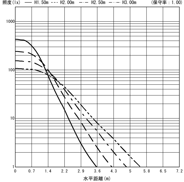
○直射水平面照度 (全光束: 1870 × 1 = 1870lm/台)
