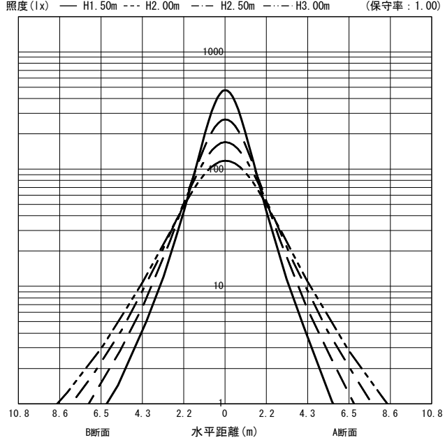
○直射水平面照度 (全光束: 2960 × 1 = 2960lm/台)
