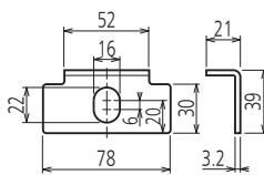
FWL型座金 (同梱部品)
