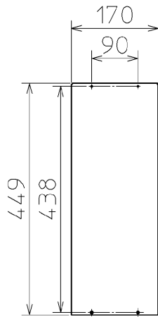
② HOOD R 007HH
