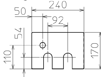
⑥ HOOD A 007HH
