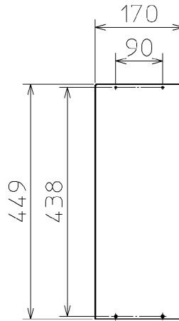
③ HOOD L 007HH
