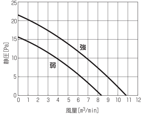
MPS-RP140KA
