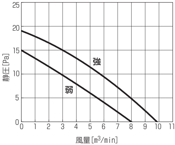
MPS-RP112KA
