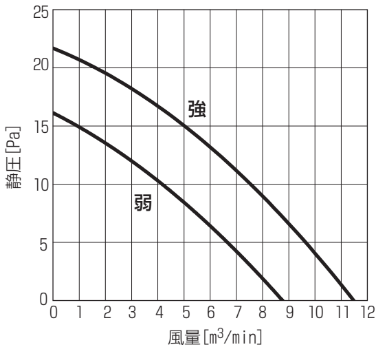
MPS-RP160KA
