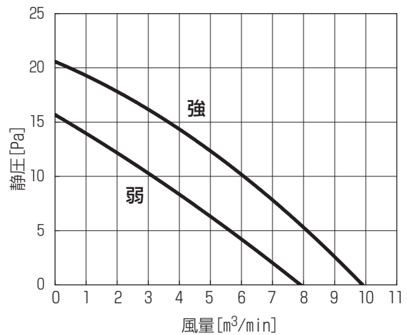
MPS-RP112GA(H)2
