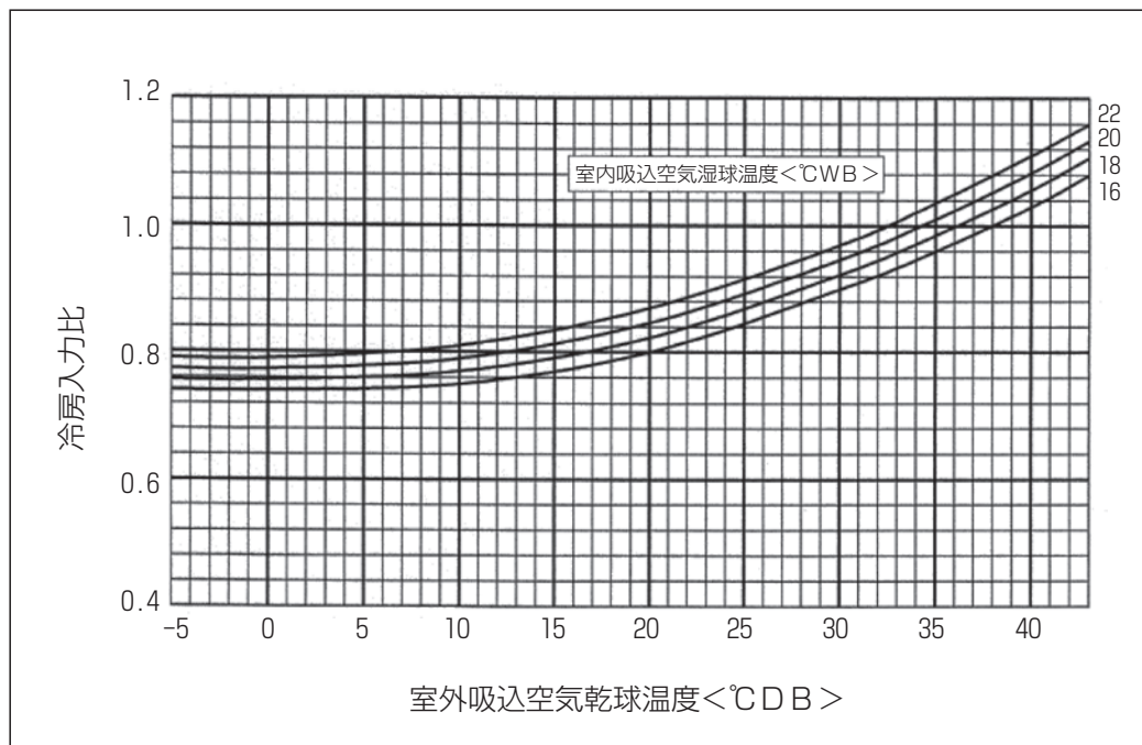
■冷房入力線図 MPUZ-ERP・HA7 / KA, MPU(Z)-RP・HA7
