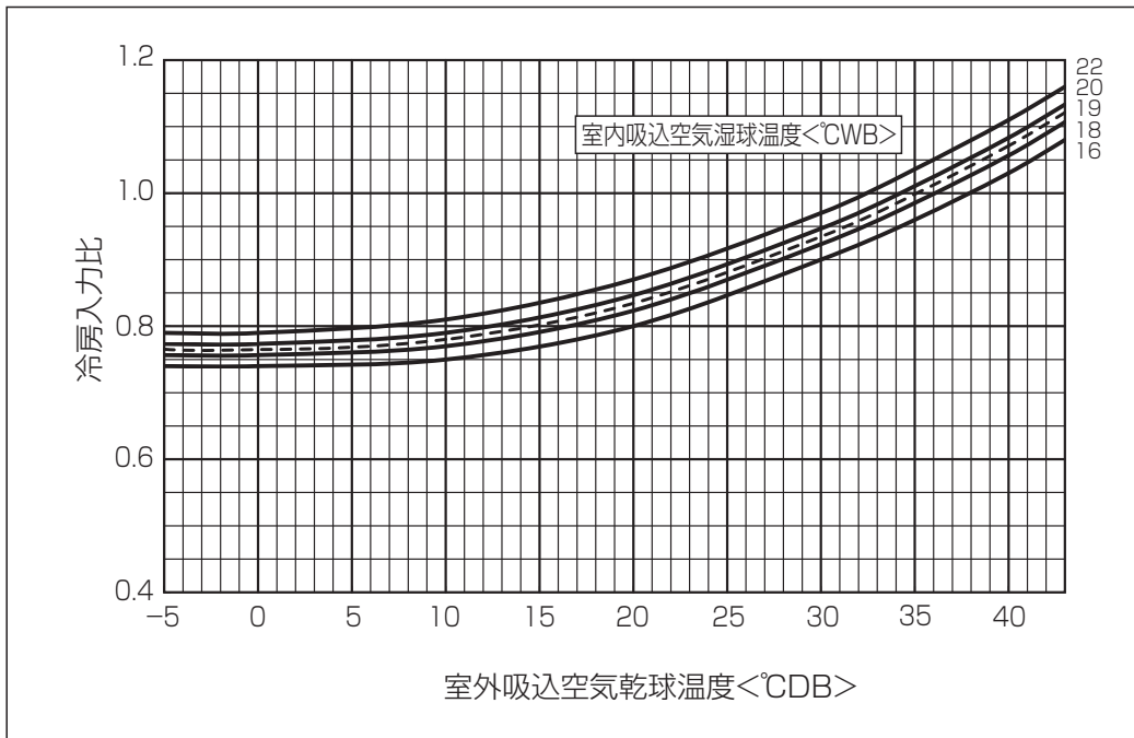
■冷房入力線図 PUZ-ZRP・KA3 / HA9, PUZ-ERP・KA3 / HA9, PU(Z)-RP・HA9
