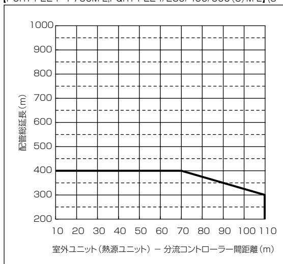
【PURY-P224~P730M-E,PQRY-P224/280/450/560(S)M-E】(8~26HP)
