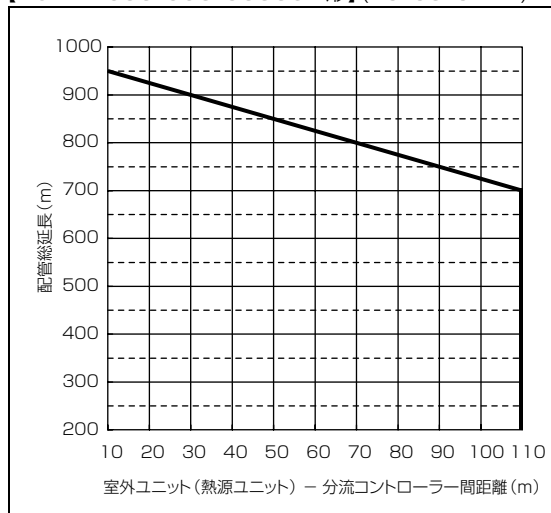
【PURY-P800/850/900SCM形】(28/30/32HP)
