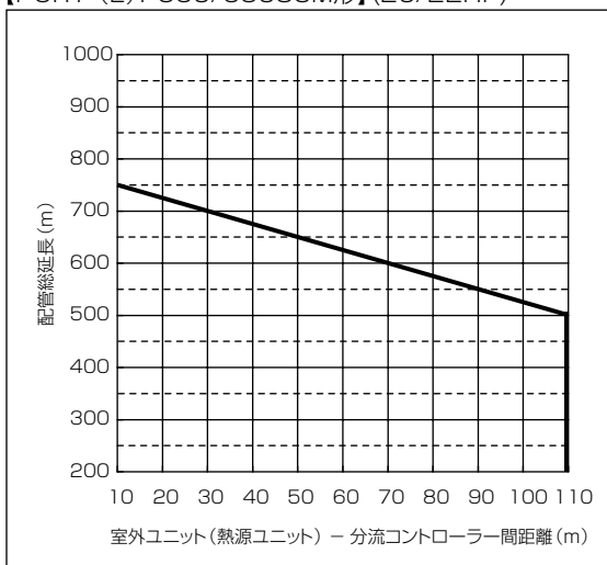
【PURY-(E)P560/630SCM形】(20/22HP)
