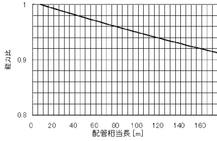
■ PURY-P224CM-E (-BS, -BSG)
