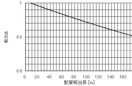
■ PURY-P800,850,900SCM-E (-BS, -BSG)
