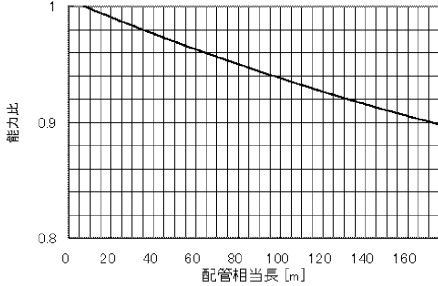
■ PURY-P450CM-E (-BS, -BSG)
