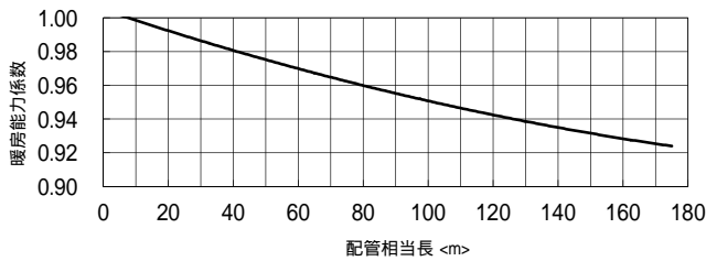
(5) P1250-F形
