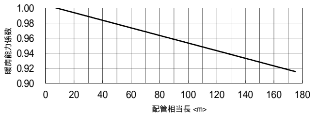
(4) P1000-F形
