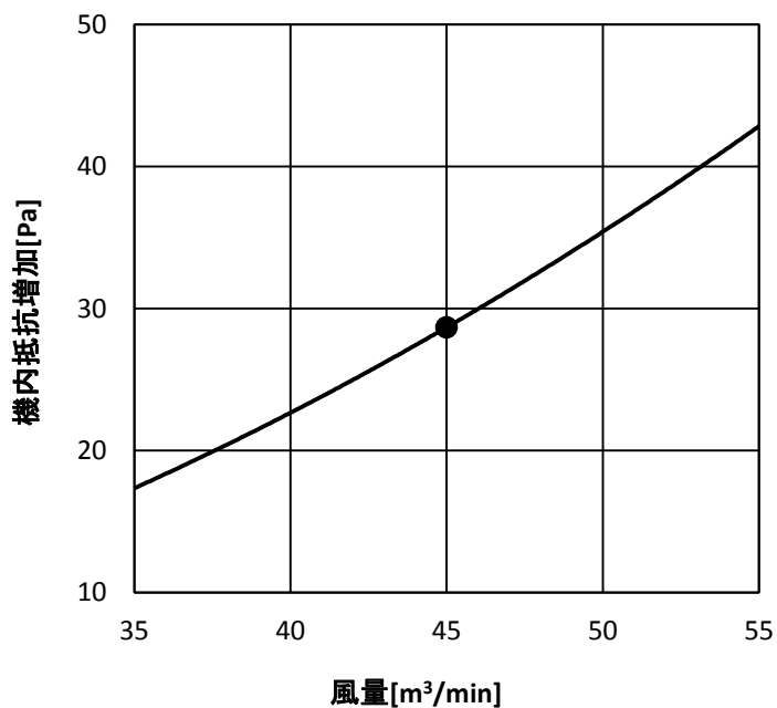
・PFAV-P140DMJ1
