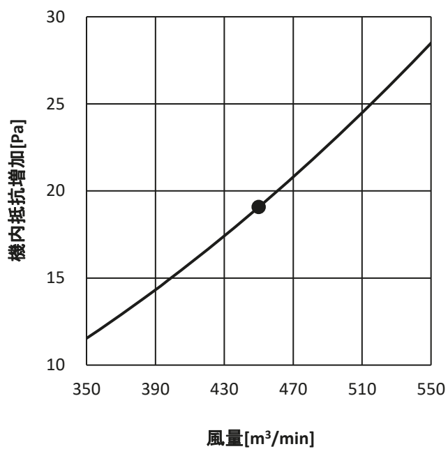
・PFAV-P1400DMJ3
