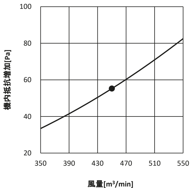
・PFAV-P1400DMJ3
